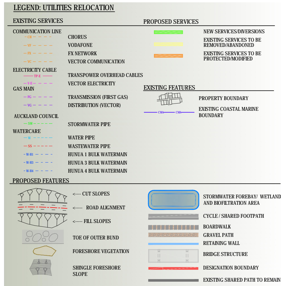
UTILITIES RELOCATION PLANS, REFER DRAWINGS AEE-U-101 TO AEE-U-116
