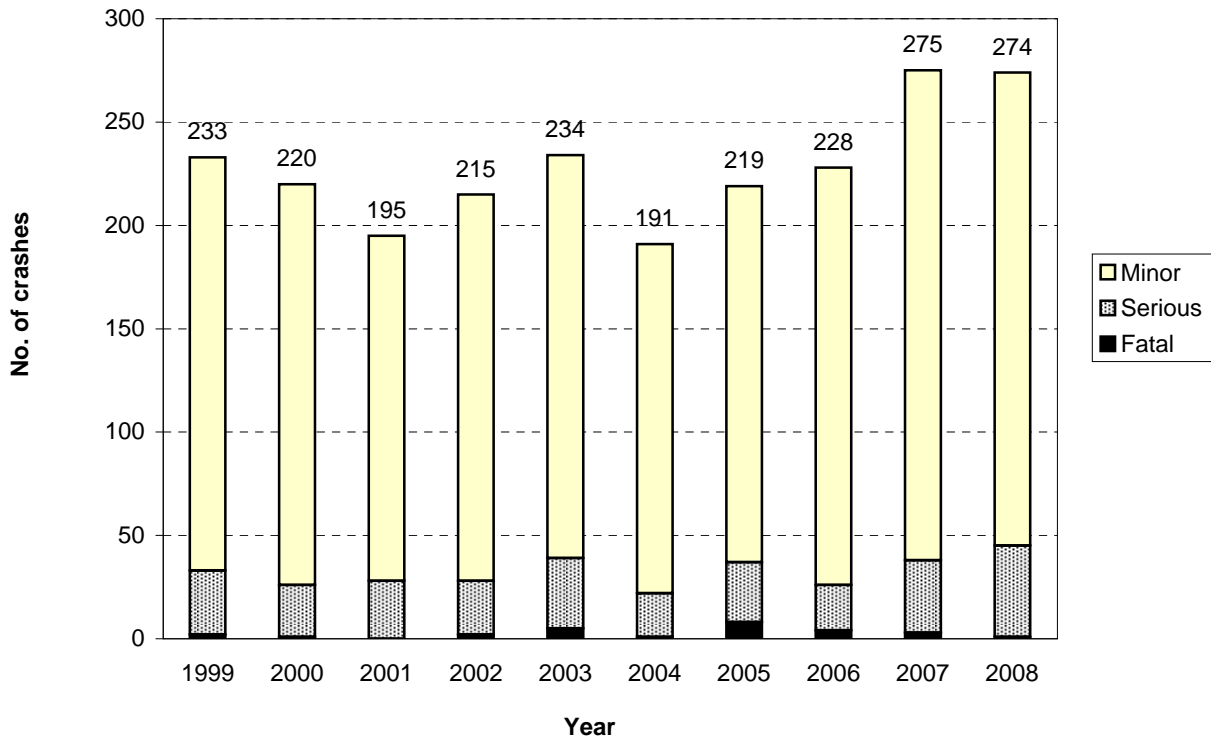
Figure 8.3 Number of injury crashes Hamilton City - urban council roads
