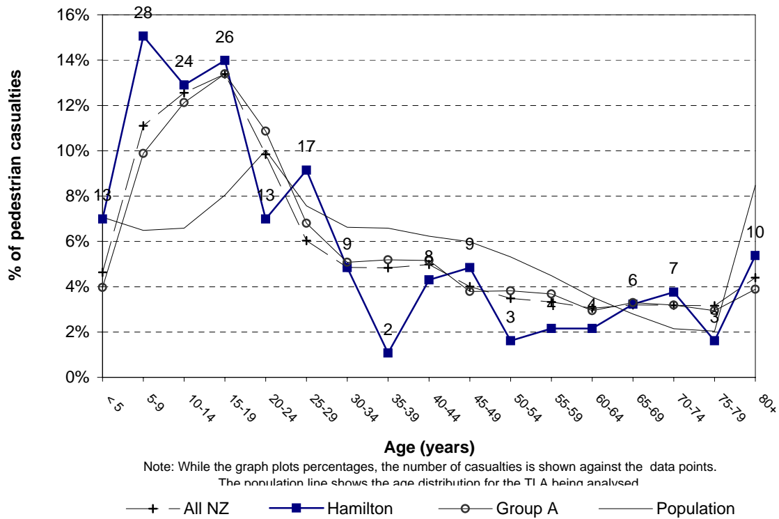
Figure 3.23 Pedestrian casualty age Hamilton City (2004-2008)
