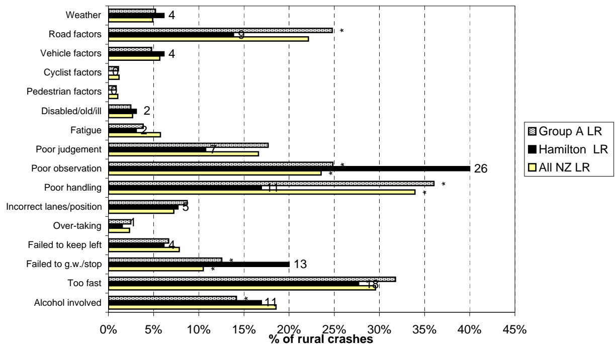
Figure 8.14 Contributing factors - rural Hamilton City council roads (2004-2008)
