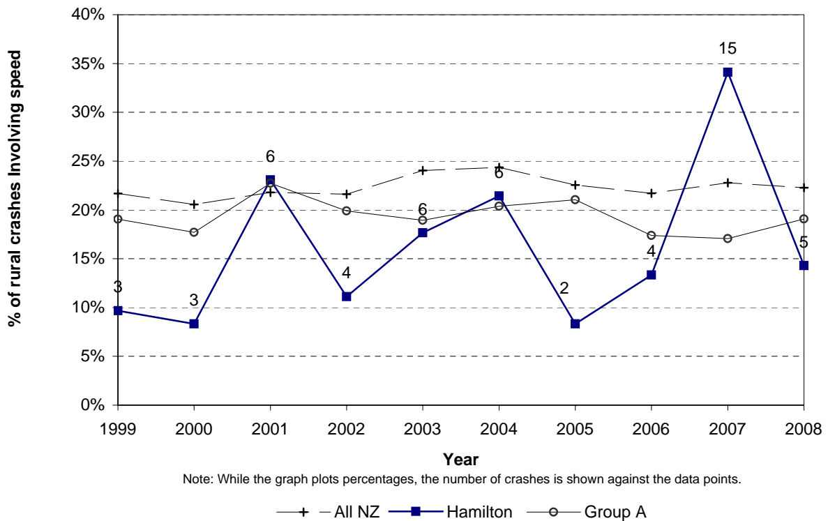
Figure 5.14 Speed involved trend Hamilton City - rural roads
