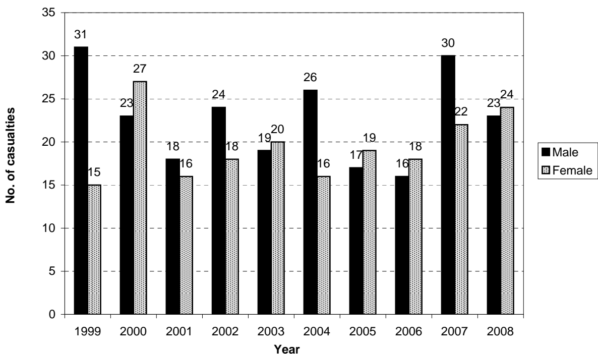
Figure 3.4 Male/female casualties - rural Hamilton City
