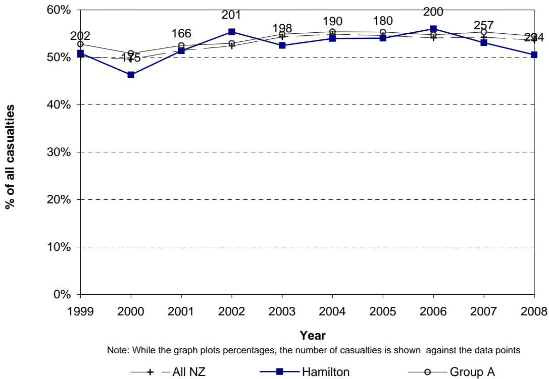
Figure 3.7 Car/van driver casualties Hamilton City
