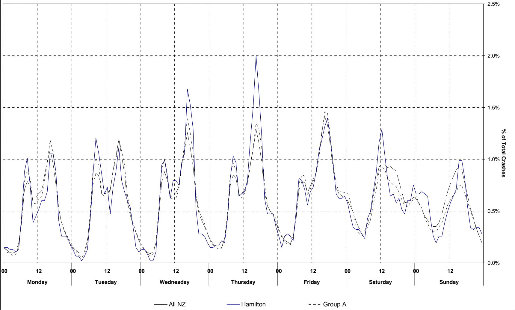
Figure 7.1 Time pattern over average week Hamilton City (2004-2008)
