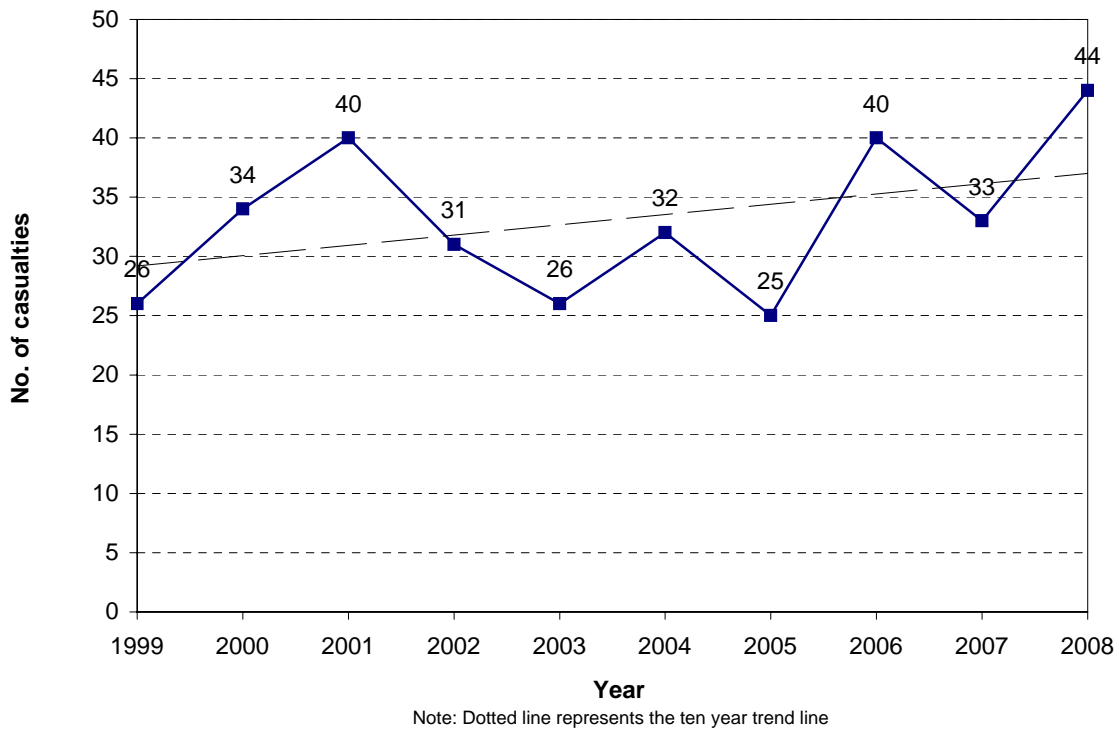
Figure 3.18 Cyclist casualties Hamilton City
