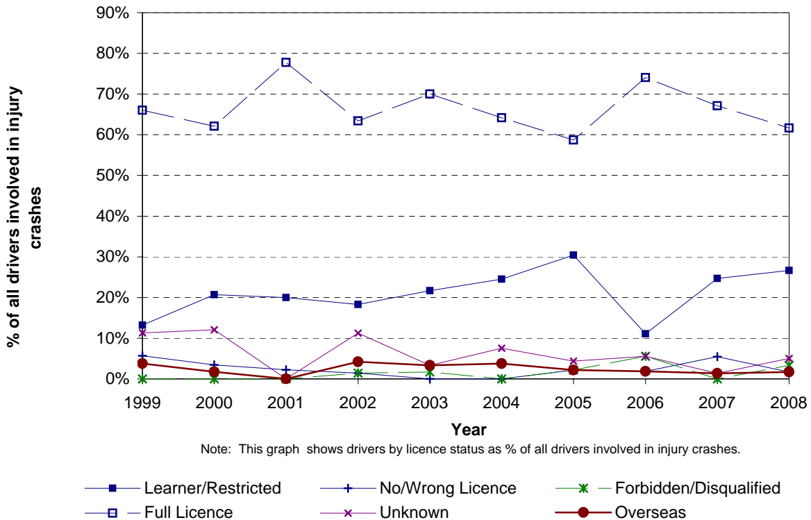
Figure 3.28 Licence status - rural Hamilton City
