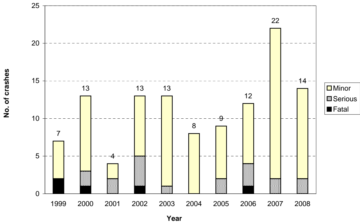
Figure 8.5 Number of injury crashes Hamilton City - rural council roads
