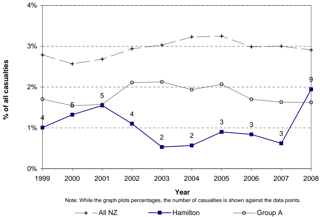
Figure 3.11 Heavy vehicle casualties Hamilton City
