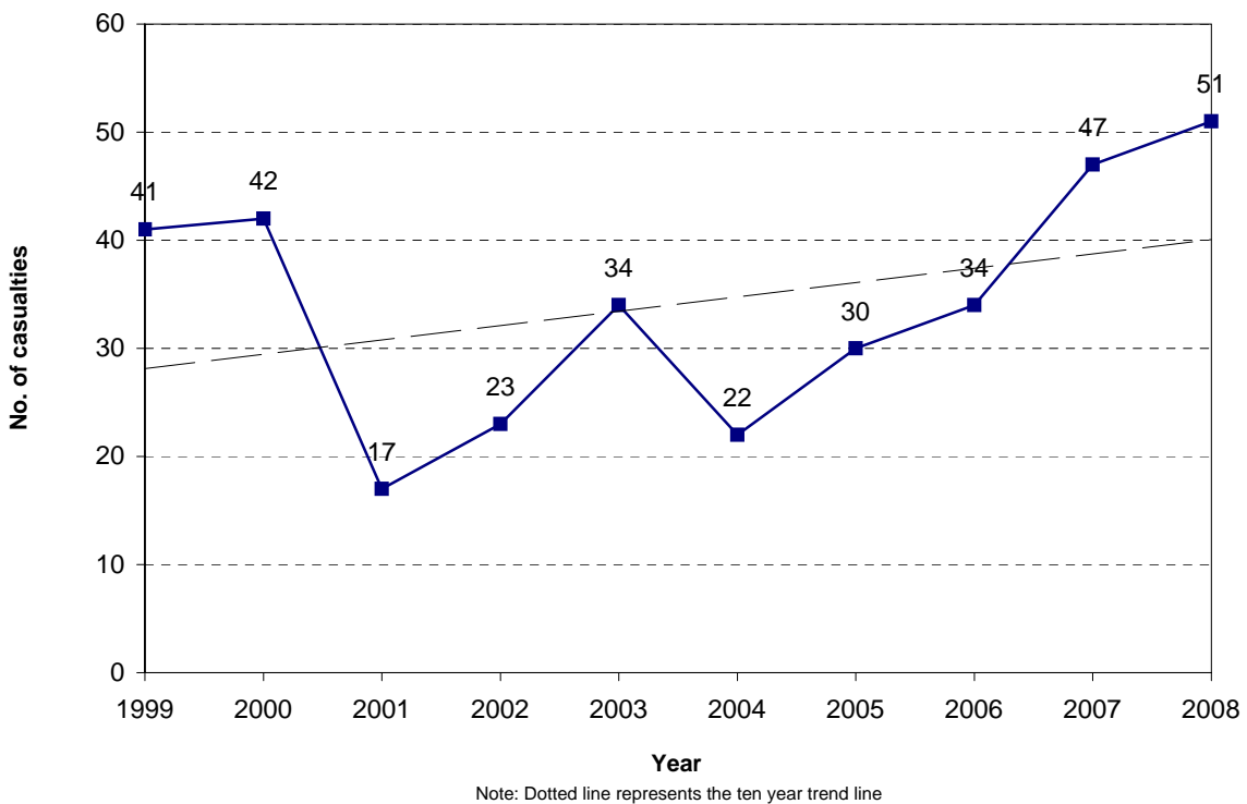
Figure 3.14 Motorcyclist casualties Hamilton City
