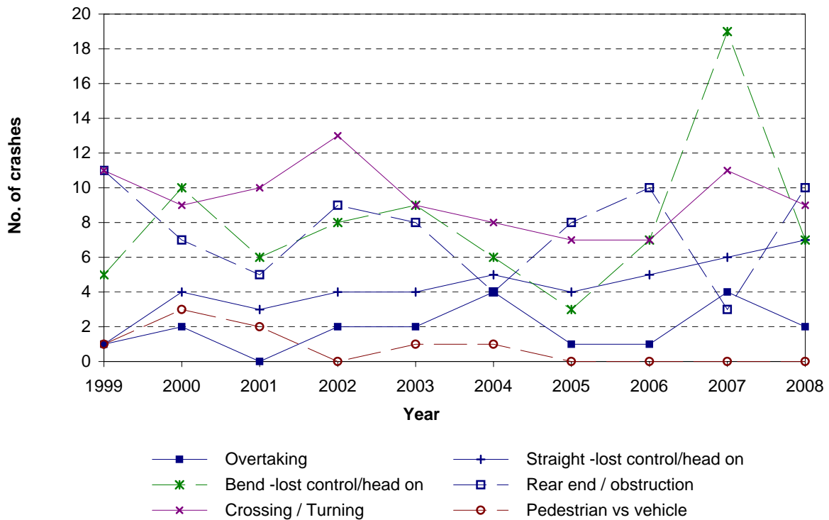
Figure 4.4 Crash movement type - trends Hamilton City - rural roads
