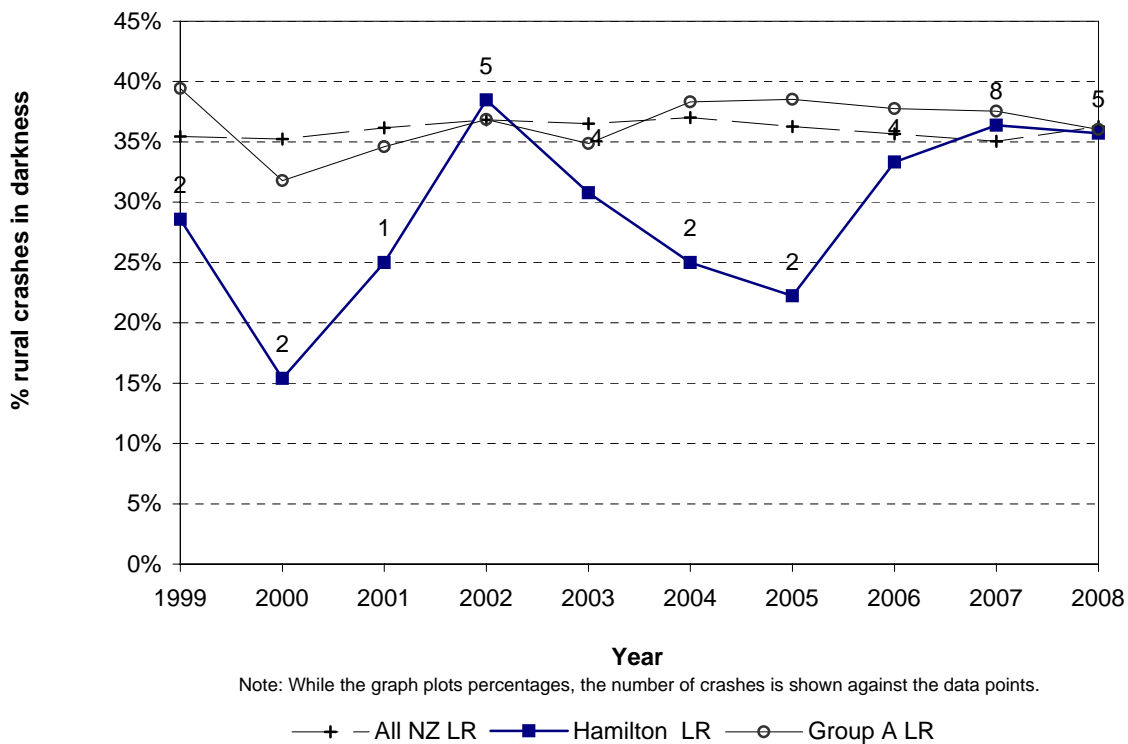
Figure 8.20 Crashes in darkness Hamilton City - rural council roads
