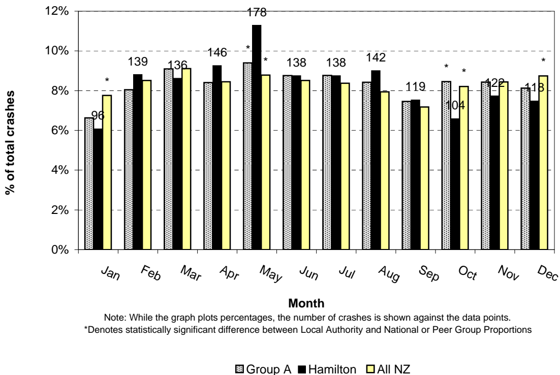
Figure 7.3 Month of year Hamilton City (2004-2008)
