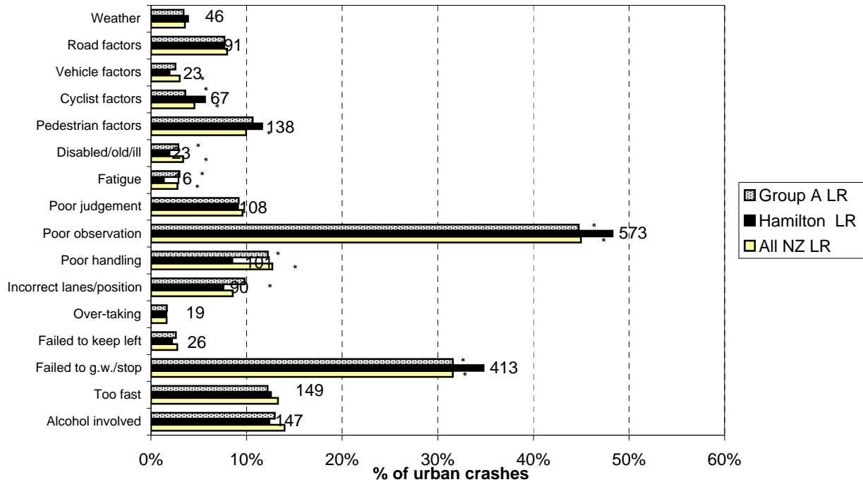
Figure 8.13 Contributing factors - urban Hamilton City council roads (2004-2008)
