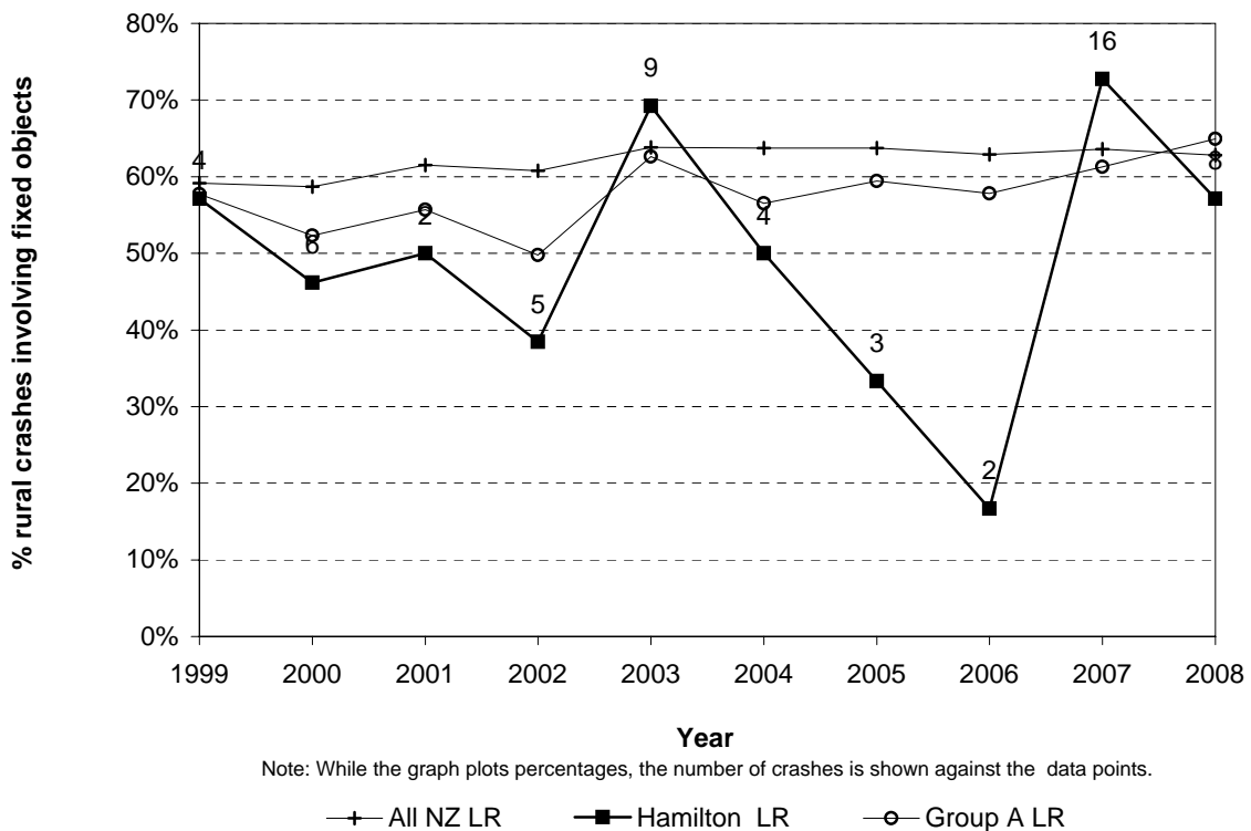
Figure 8.24 Collisions with objects Hamilton City - rural council roads
