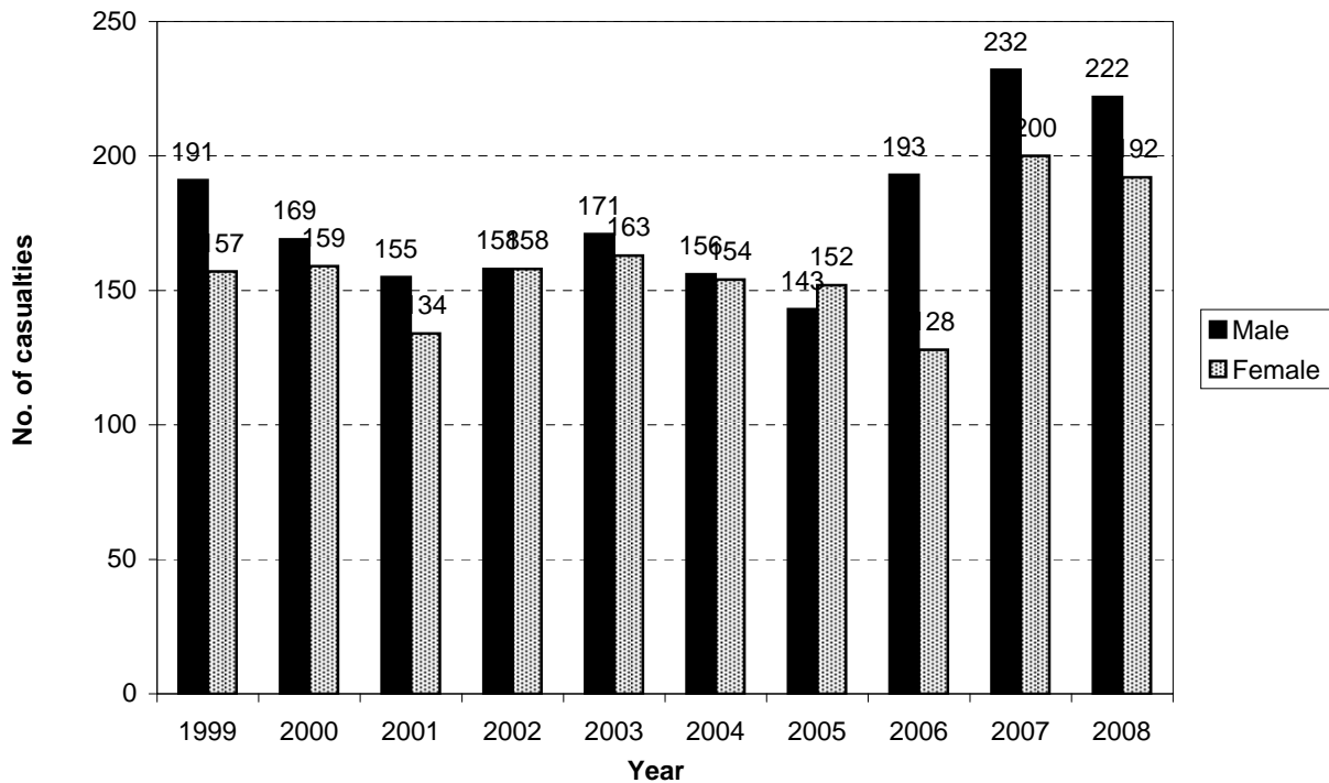
Figure 3.3 Male/female casualties - urban Hamilton City
