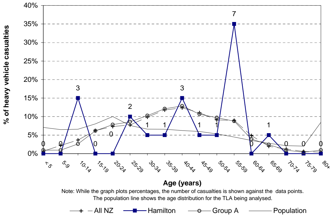
Figure 3.21 Heavy vehicle casualty age Hamilton City (2004-2008)
