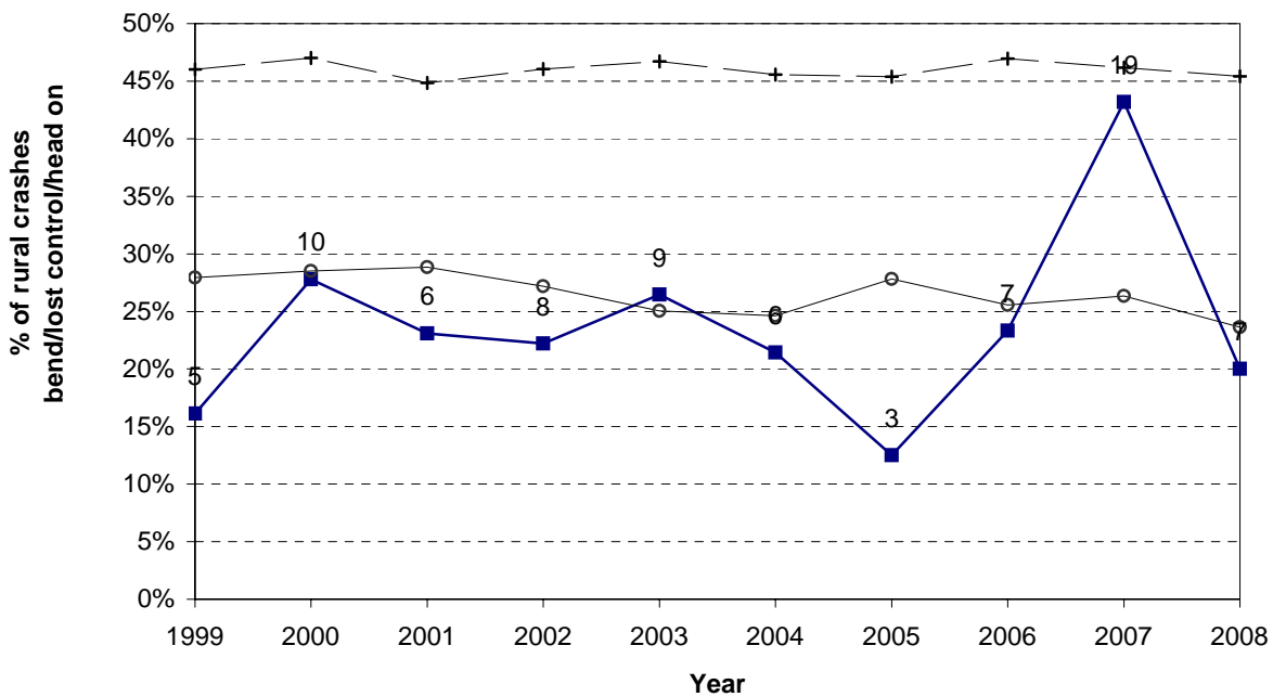
Figure 4.6 Bend - lost control / head - on Hamilton City - rural roads
