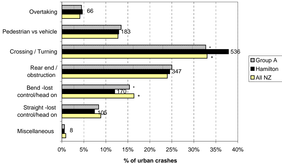
Figure 4.1 Crash movement type - urban Hamilton City (2004-2008)
