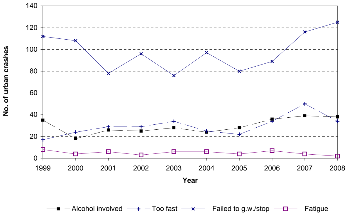
Figure 5.3 Contributing factor trends Hamilton City - urban roads
