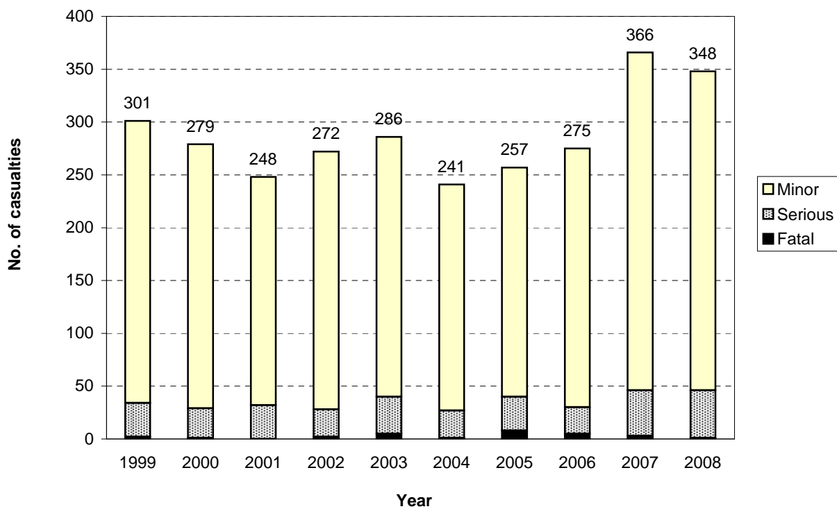
Figure 8.4 Number of casualties Hamilton City - urban council roads
