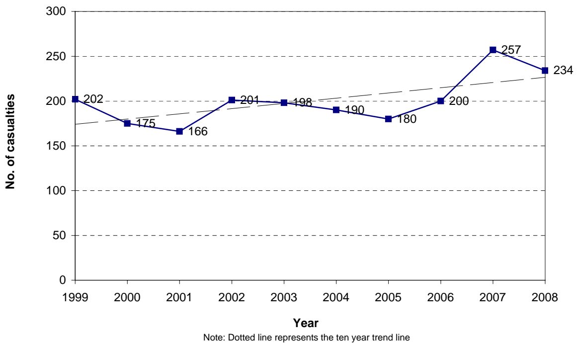
Figure 3.8 Car/van driver casualties Hamilton City
