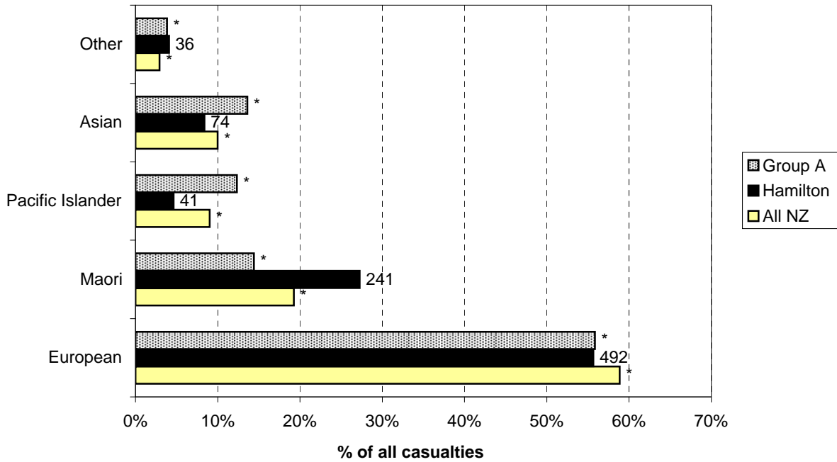
Figure 3.25 Casualty ethnicity - urban Hamilton City (2004-2008)
