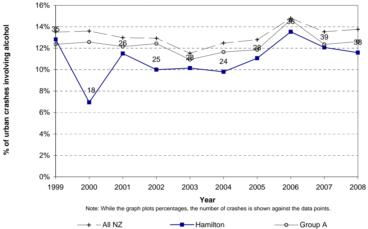
Figure 5.7 Alcohol involved trend Hamilton City - urban roads
