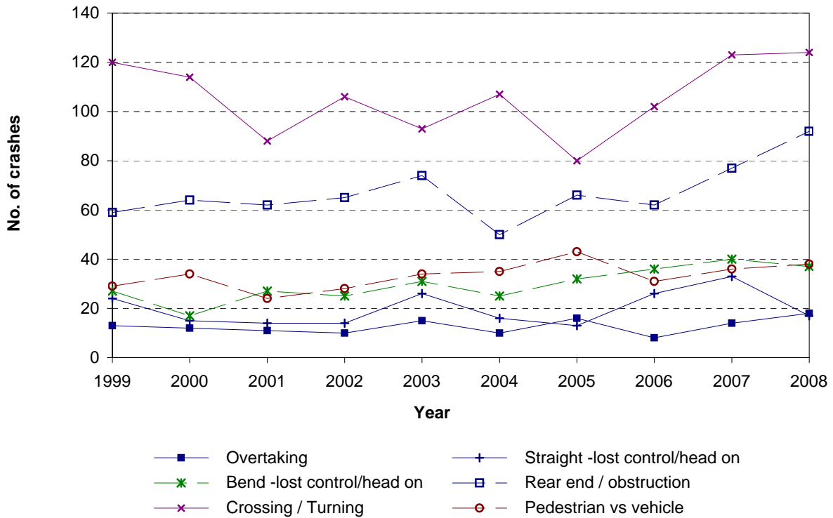
Figure 4.3 Crash movement type - trends Hamilton City - urban roads
