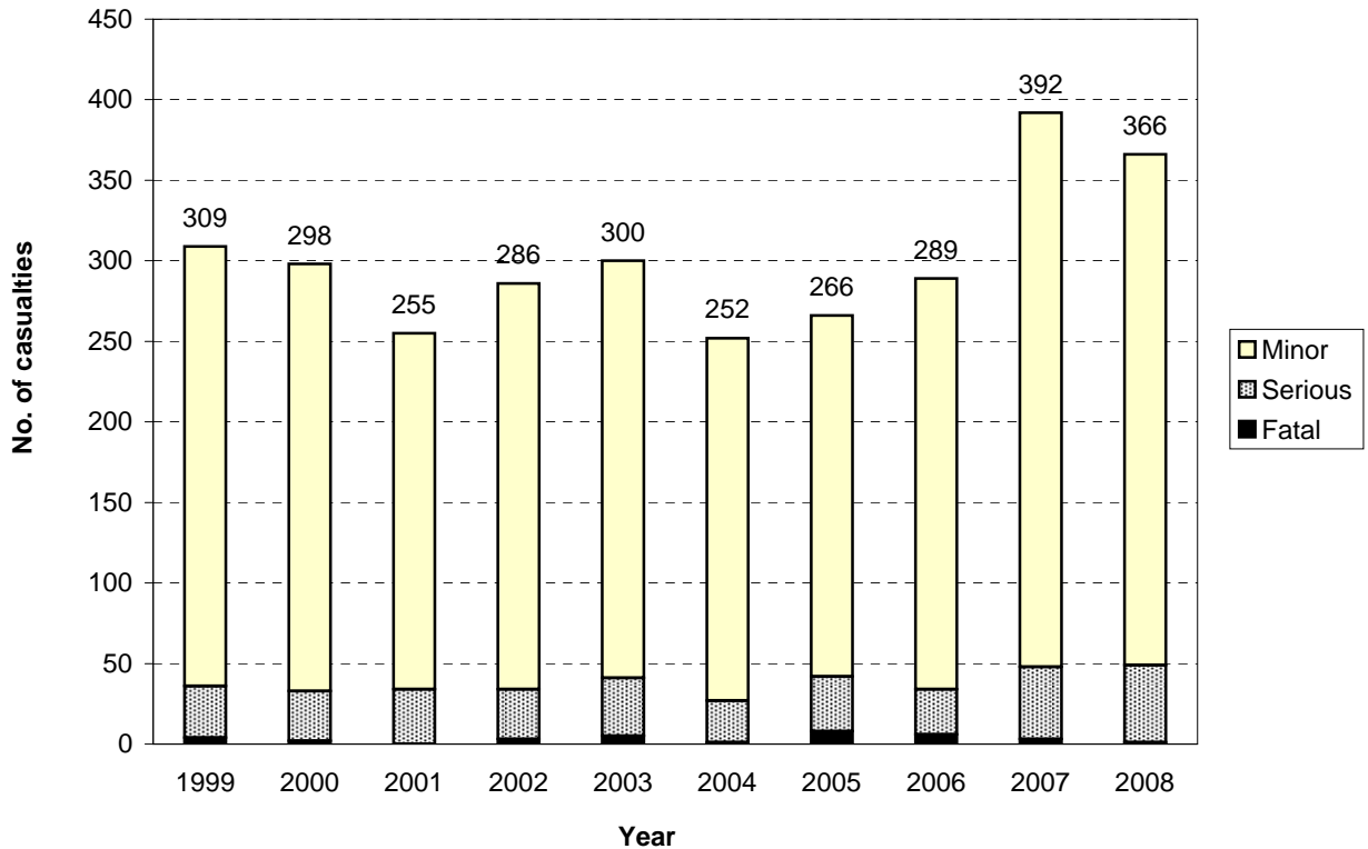
Figure 8.2 Number of casualties Hamilton City - council roads (urban & rural)
