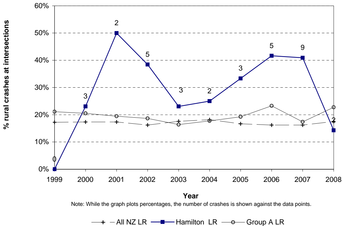
Figure 8.16 Intersection crashes Hamilton City - rural council roads
