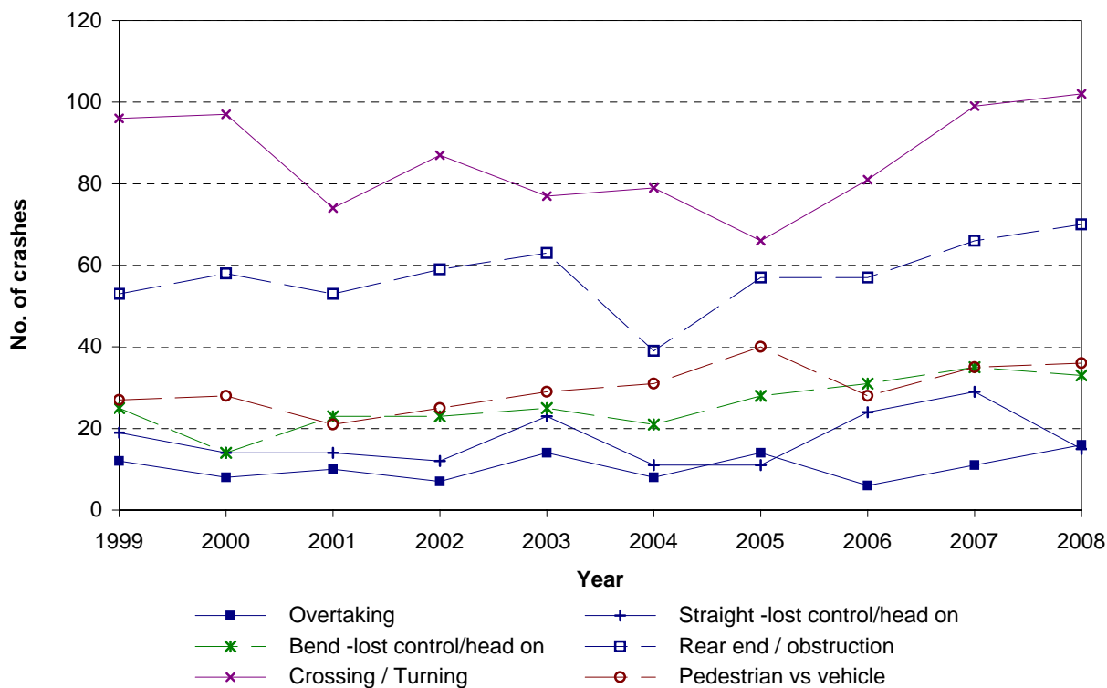
Figure 8.10 Crash movement type - Trends Hamilton City - rural council roads
