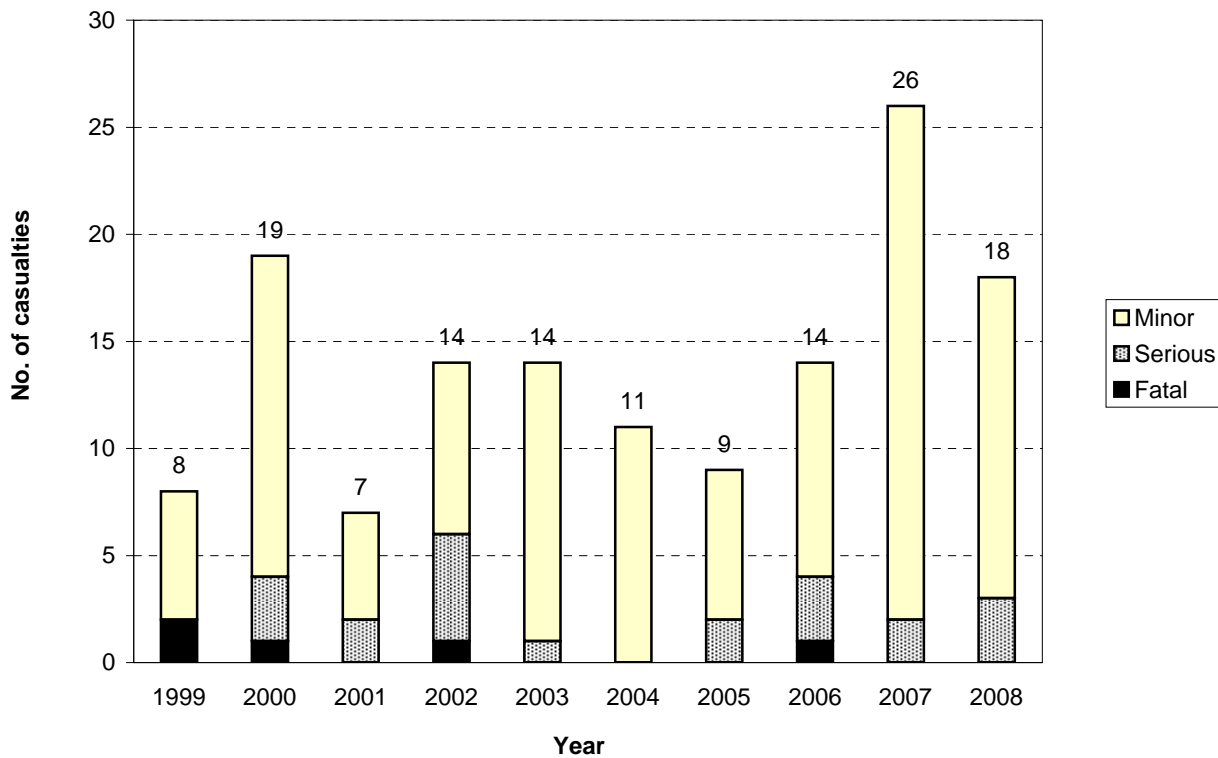
Figure 8.6 Number of casualties Hamilton City - rural council roads
