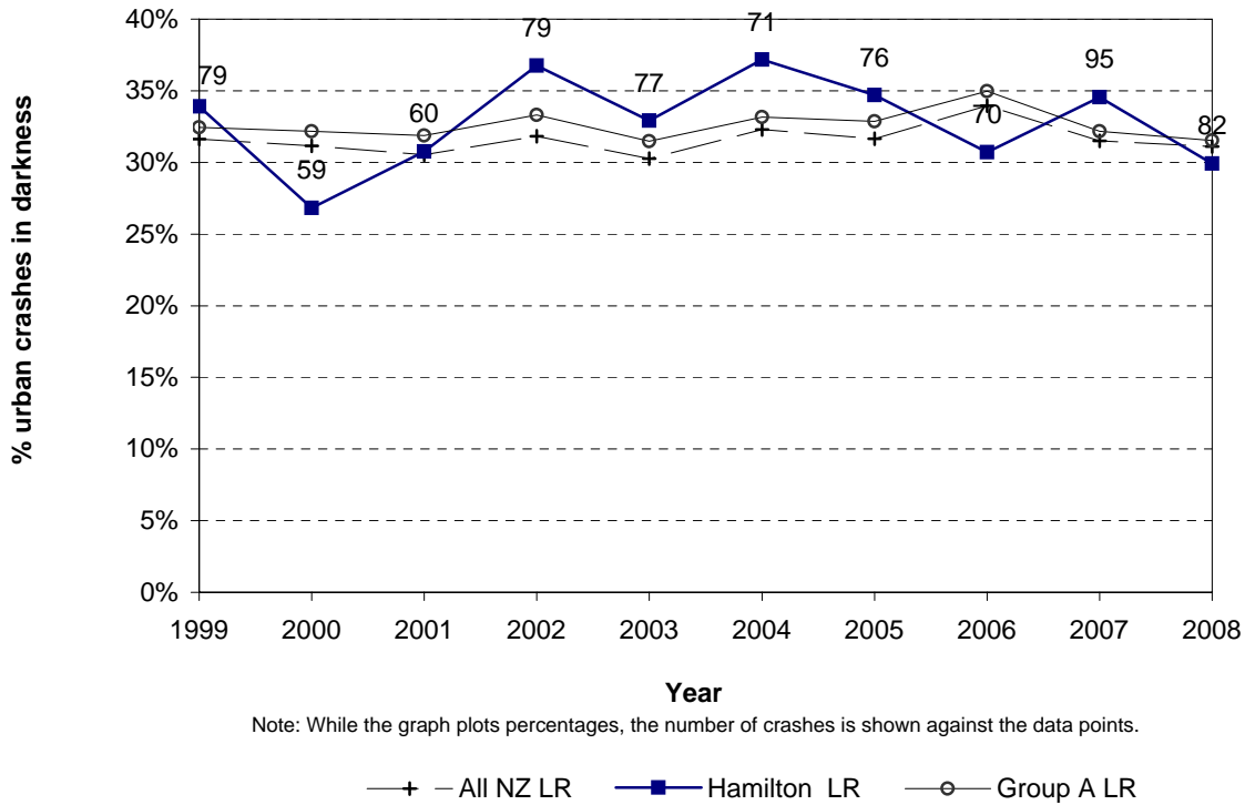
Figure 8.19 Crashes in darkness Hamilton City - urban council roads
