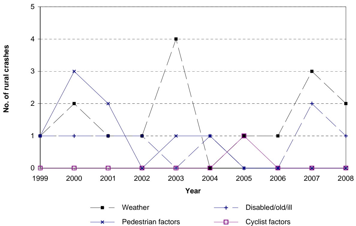
Figure 5.12 Contributing factor trends Hamilton City - rural roads
