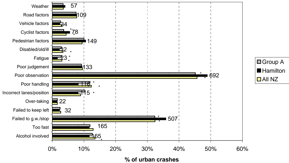
Figure 5.1 Contributing factors - urban Hamilton City (2004-2008)
