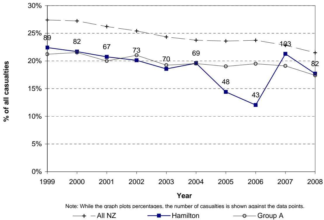
Figure 3.9 Car/van passenger casualties Hamilton City
