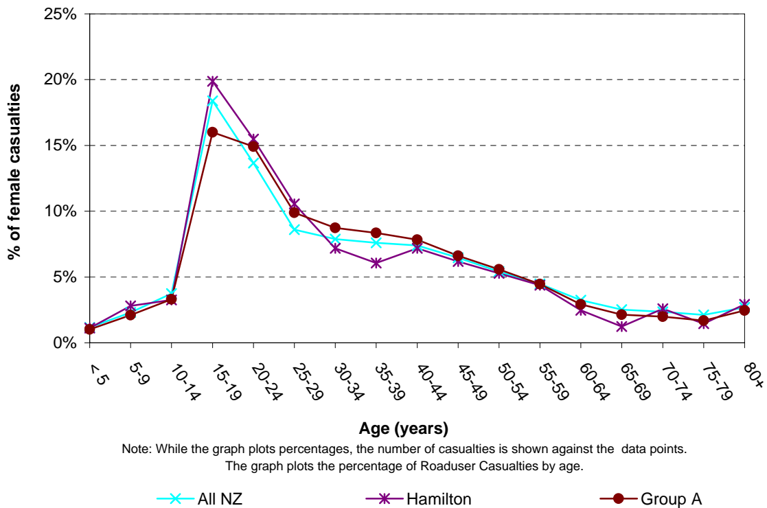
Figure 3.6 Female casualties by age Hamilton City (2004-2008)
