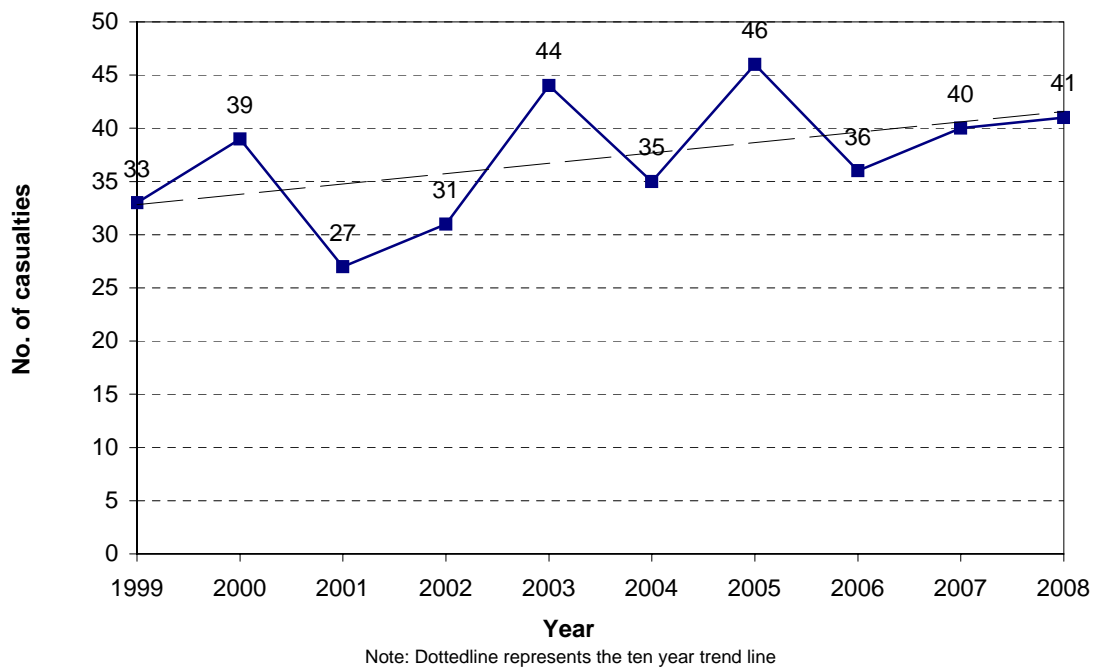
Figure 3.16 Pedestrian casualties Hamilton City
