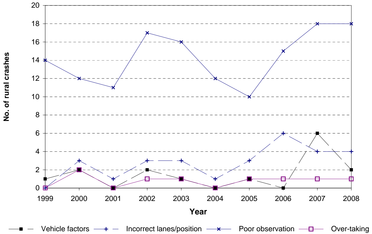
Figure 5.12 Contributing factor trends Hamilton City - rural roads
