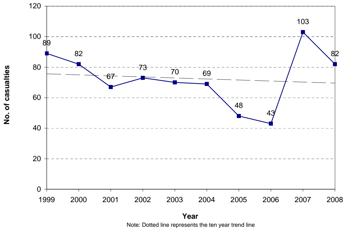
Figure 3.10 Car/van passenger casualties Hamilton City
