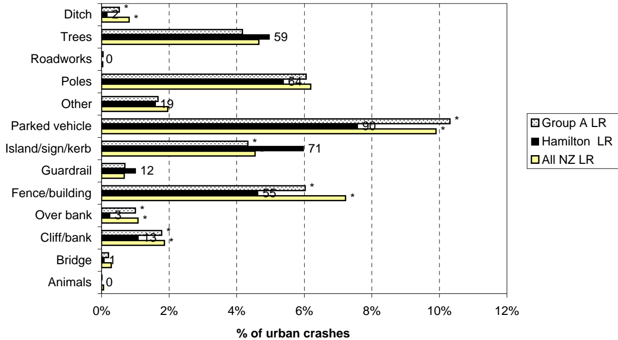
Figure 8.25 Objects struck - urban Hamilton City council roads (2004-2008)
