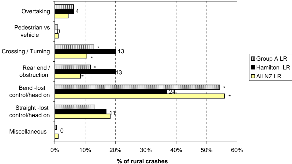
Figure 8.8 Crash movement type - rural Hamilton City council roads (2004-2008)
