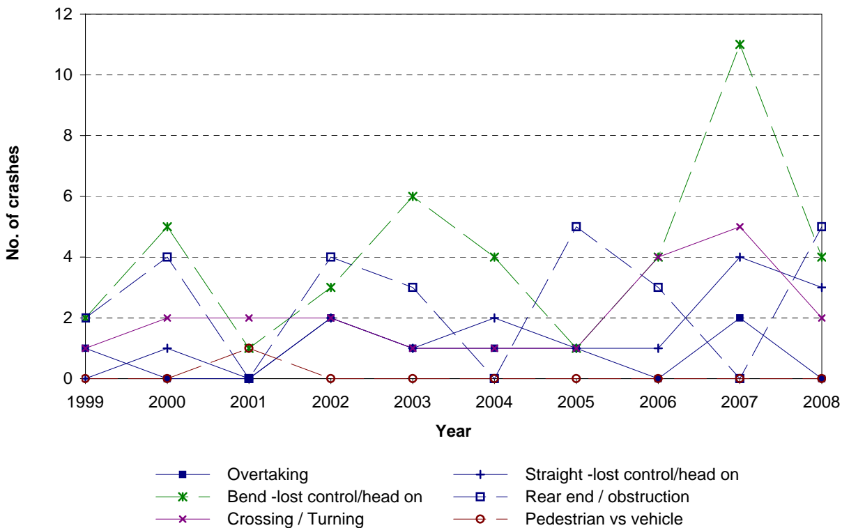
Figure 8.10 Crash movement type - Trends Hamilton City - rural council roads
