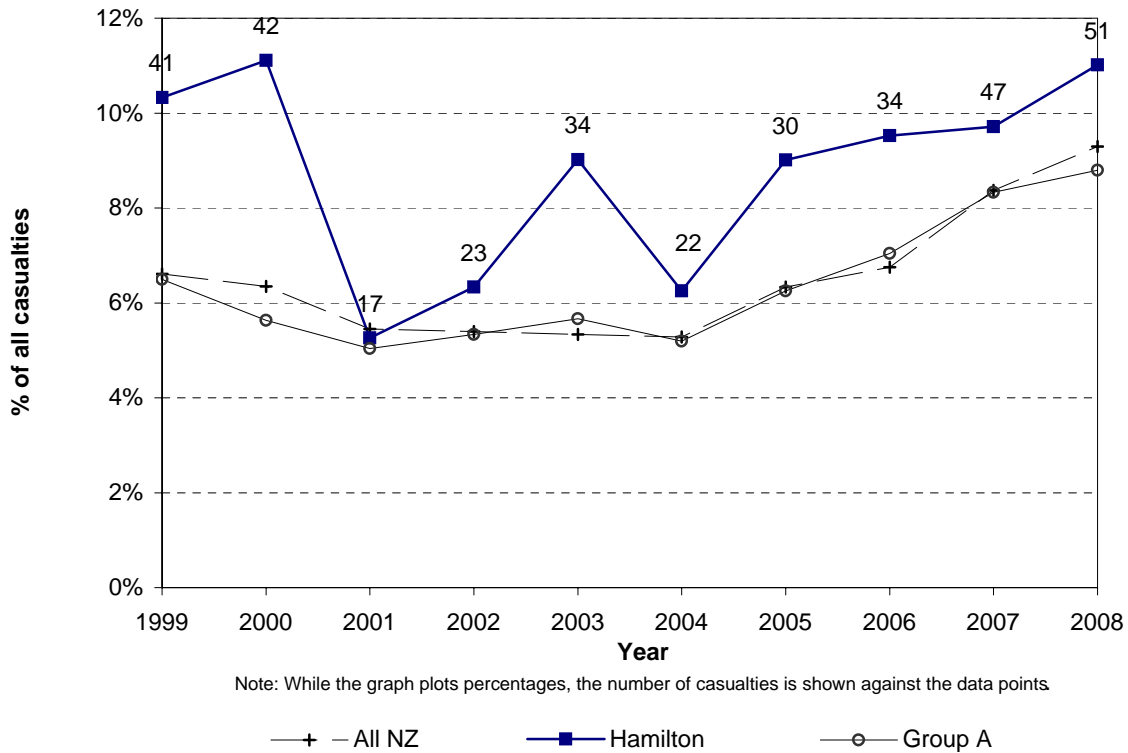
Figure 3.13 Motorcyclist casualties Hamilton City
