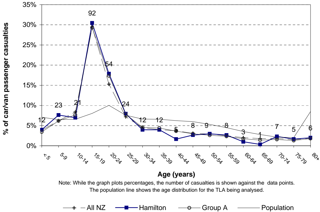
Figure 3.20 Car/van passenger casualty age Hamilton City (2004-2008)
