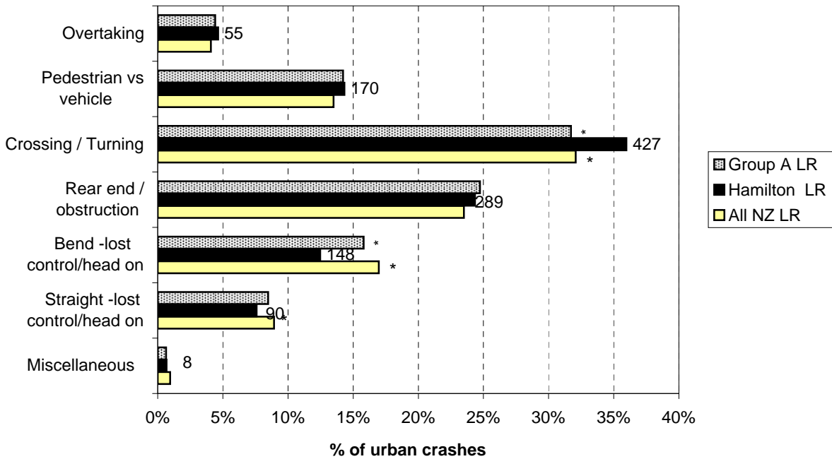
Figure 8.7 Crash movement type - urban Hamilton City council roads (2004-2008)
