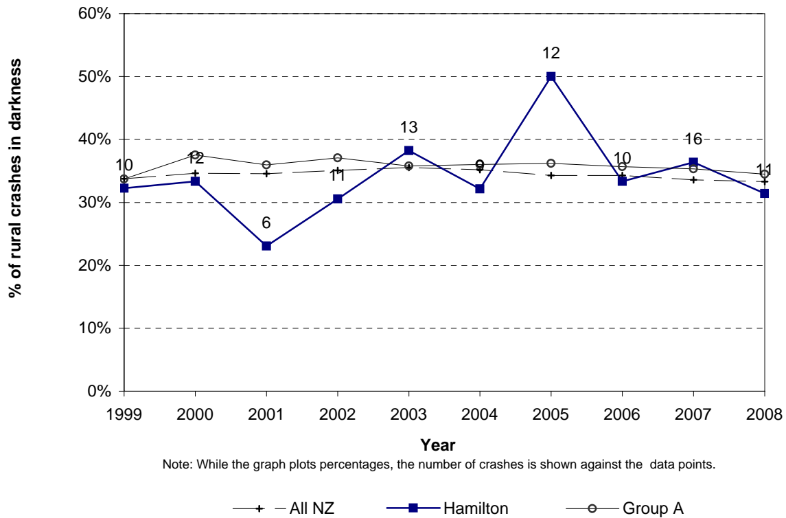
Figure 6.8 Crashes in darkness Hamilton City - rural roads
