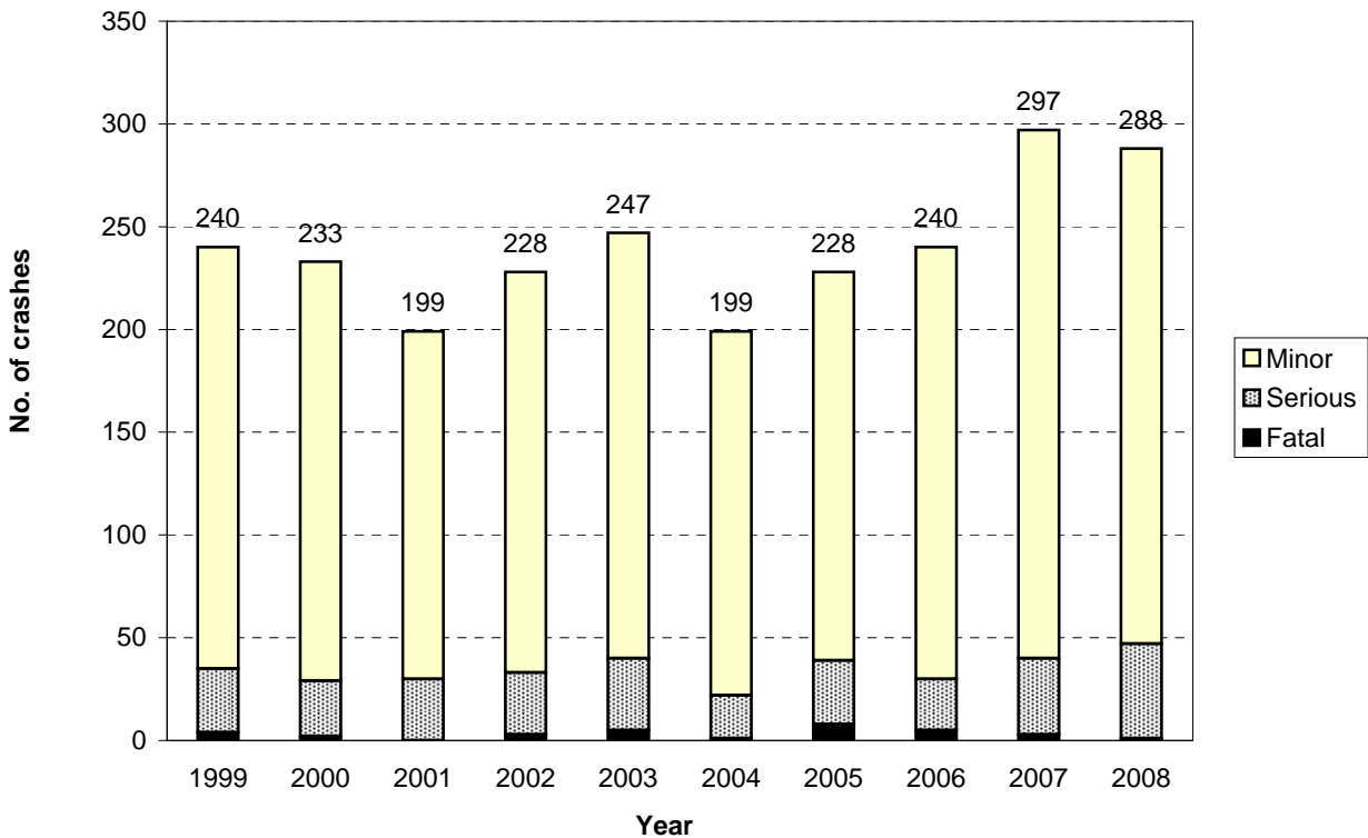
Figure 8.1 Number of injury crashes Hamilton City - council roads (urban & rural)
