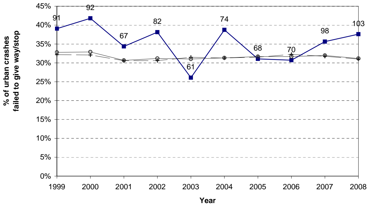
Figure 8.11 Failed to give way/stop Hamilton City - urban council roads
