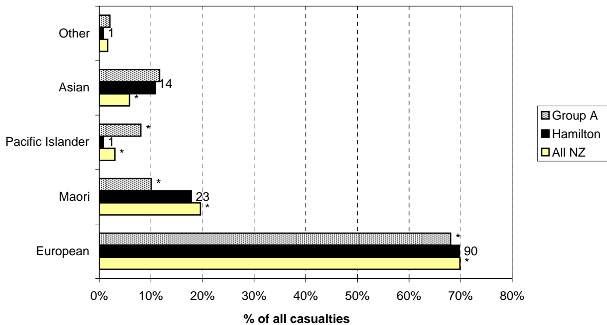
Figure 3.26 Casualty ethnicity - rural Hamilton City (2004-2008)
