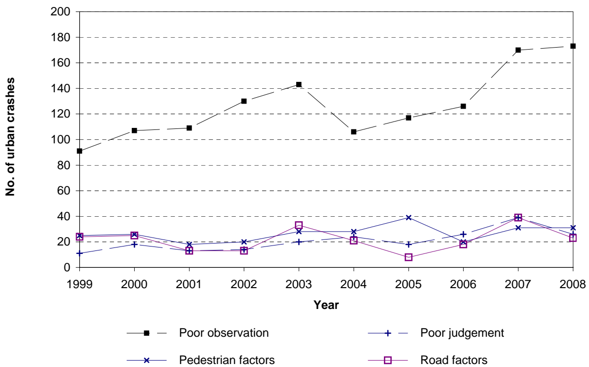
Figure 5.4 Contributing factor trends Hamilton City - urban roads
