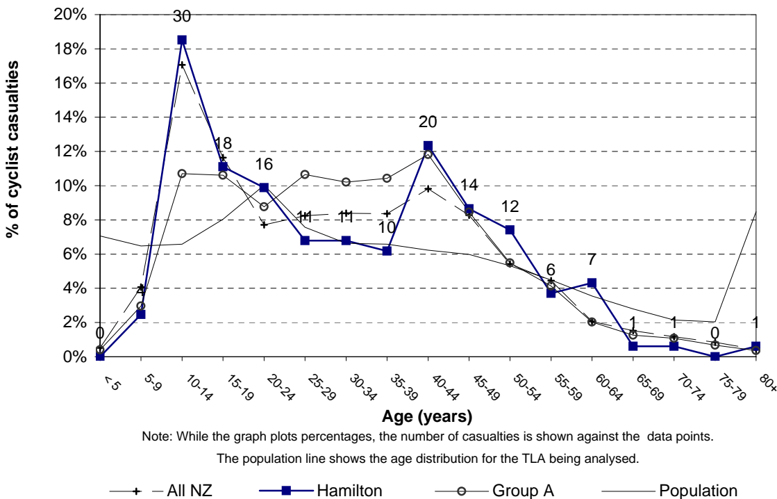
Figure 3.24 Cyclist casualty age Hamilton City (2004-2008)
