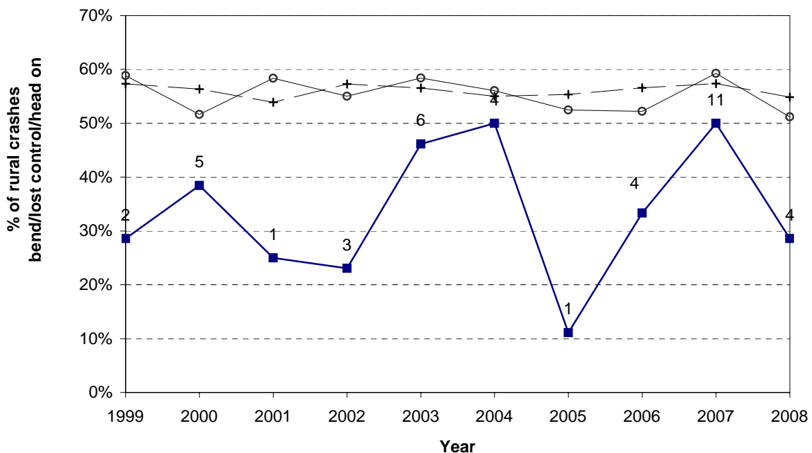
Figure 8.12 Bend - lost control / head - on Hamilton City - rural council roads
