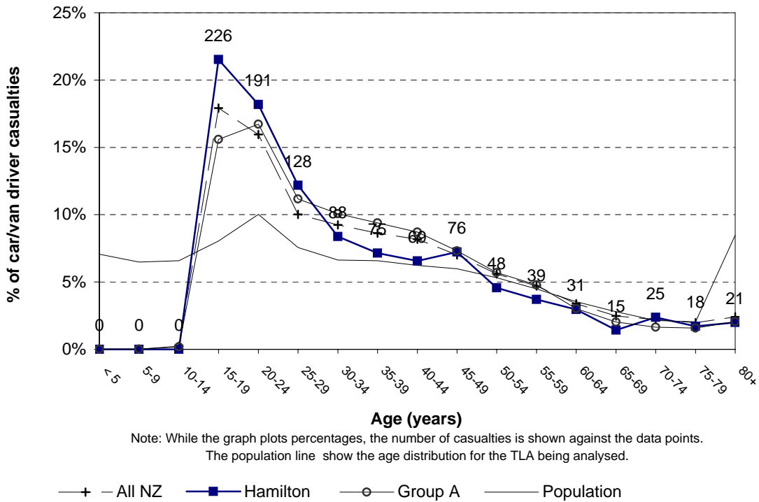
Figure 3.19 Car/van driver casualty age Hamilton City (2004-2008)
