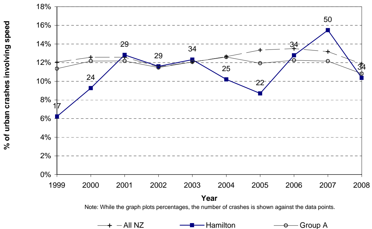
Figure 5.8 Speed involved trend Hamilton City - urban roads
