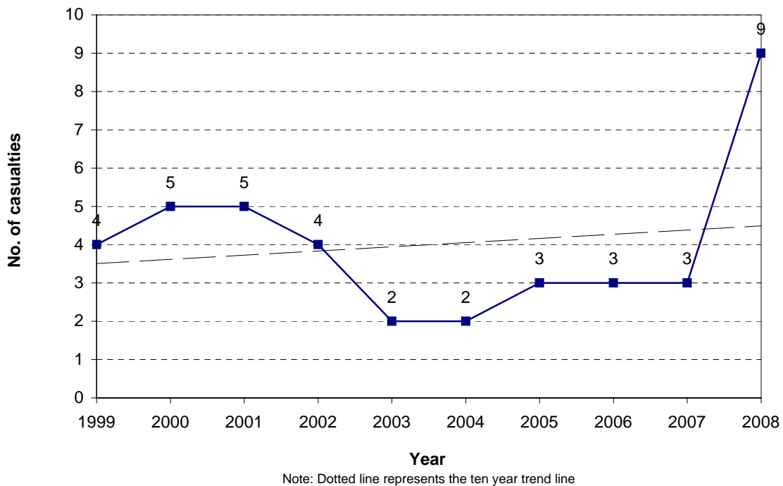
Figure 3.12 Heavy vehicle casualties Hamilton City
