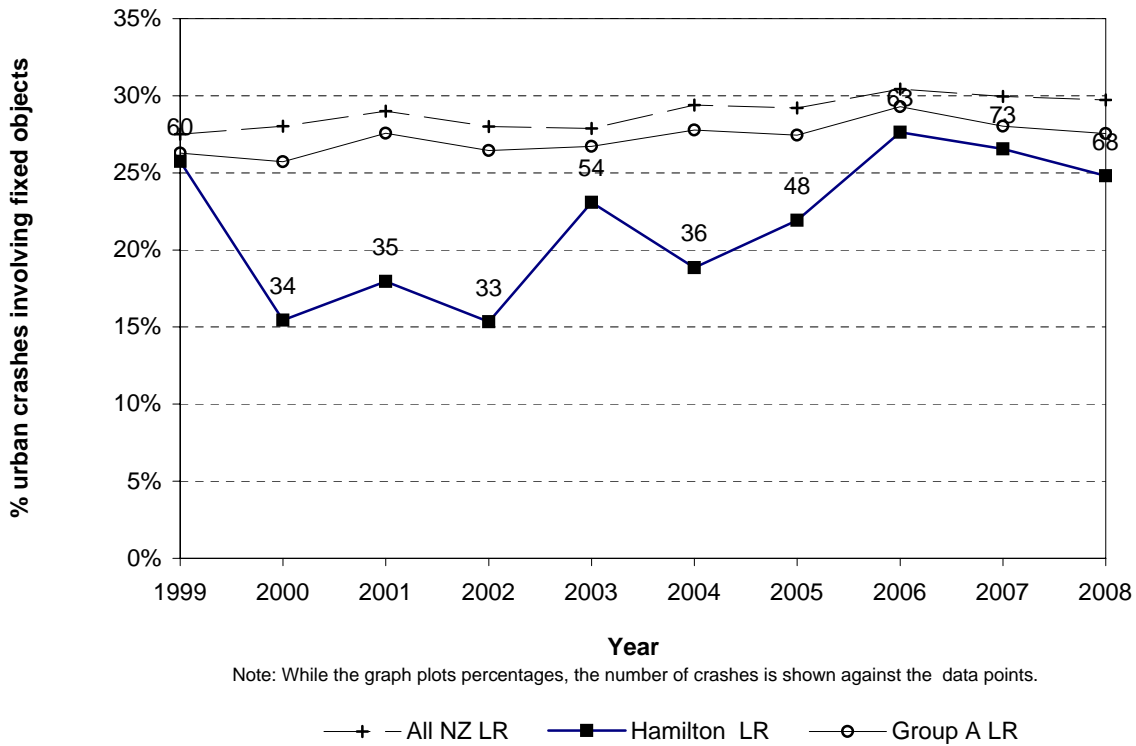
Figure 8.23 Collisions with objects Hamilton City - urban council roads
