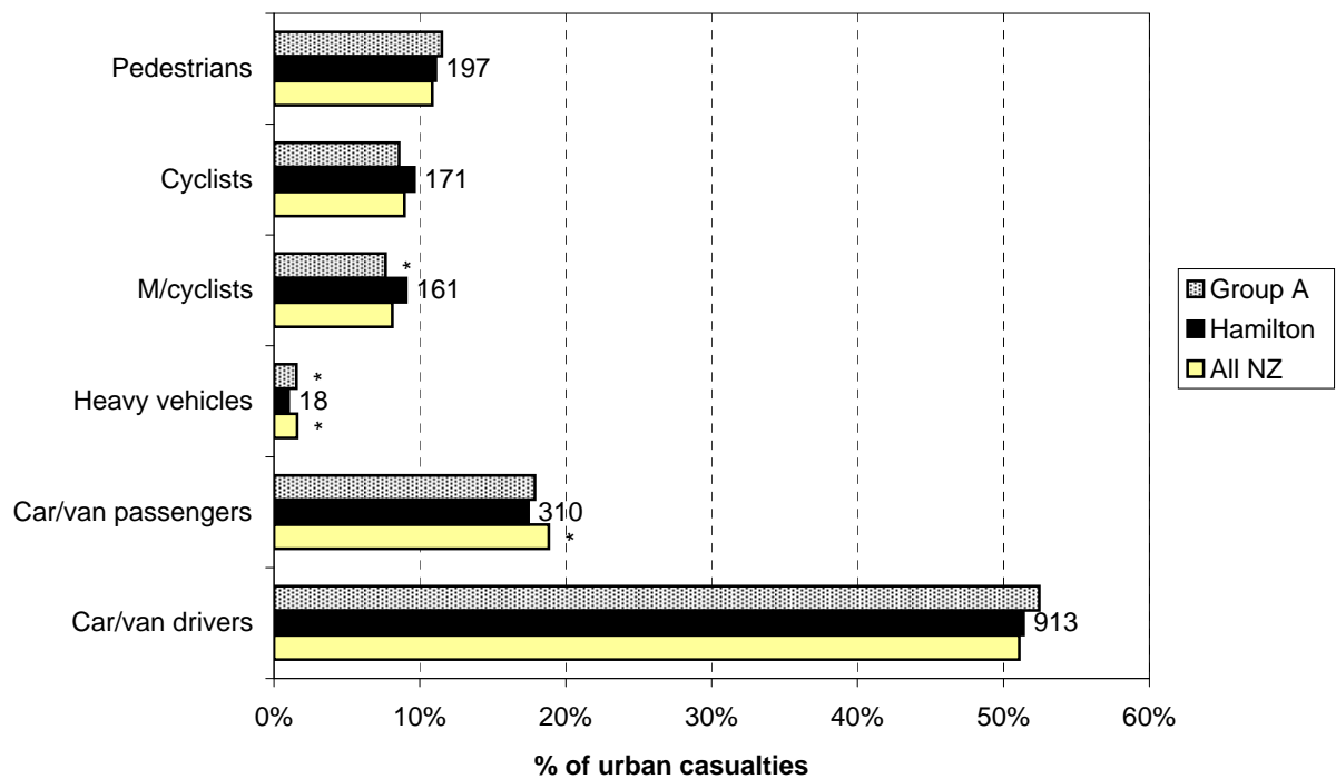
Figure 3.1 Road user casualties - urban Hamilton City (2004-2008)
