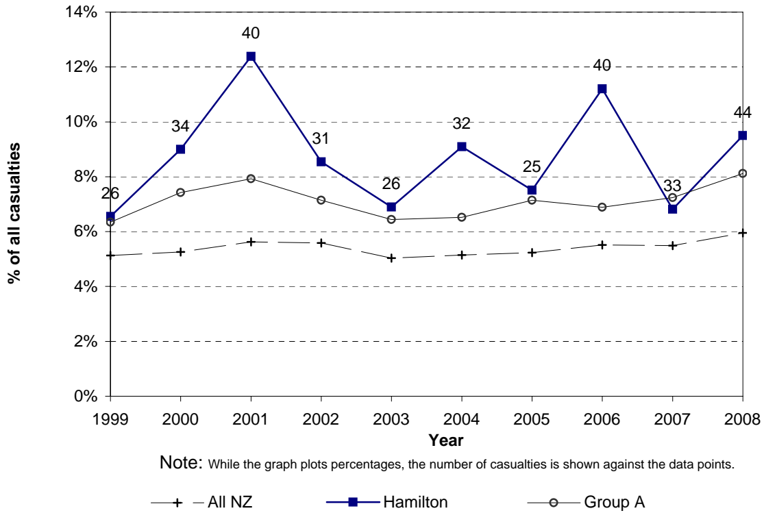
Figure 3.17 Cyclist casualties Hamilton City
