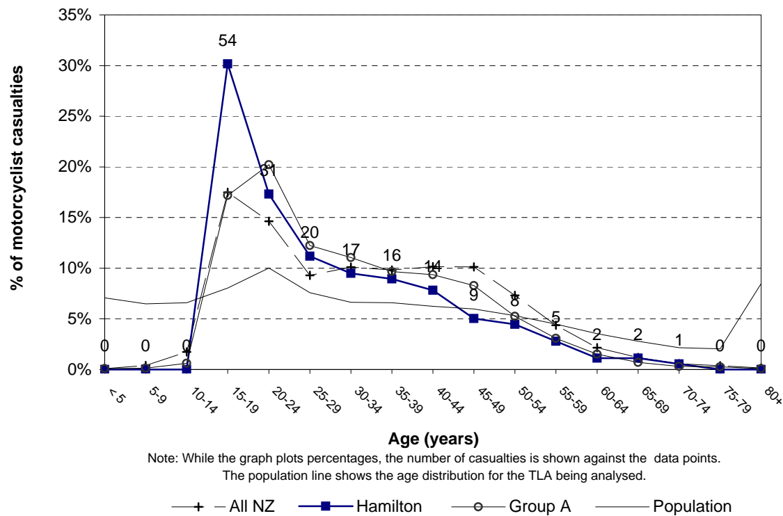
Figure 3.22 Motorcyclist casualty age Hamilton City (2004-2008)
