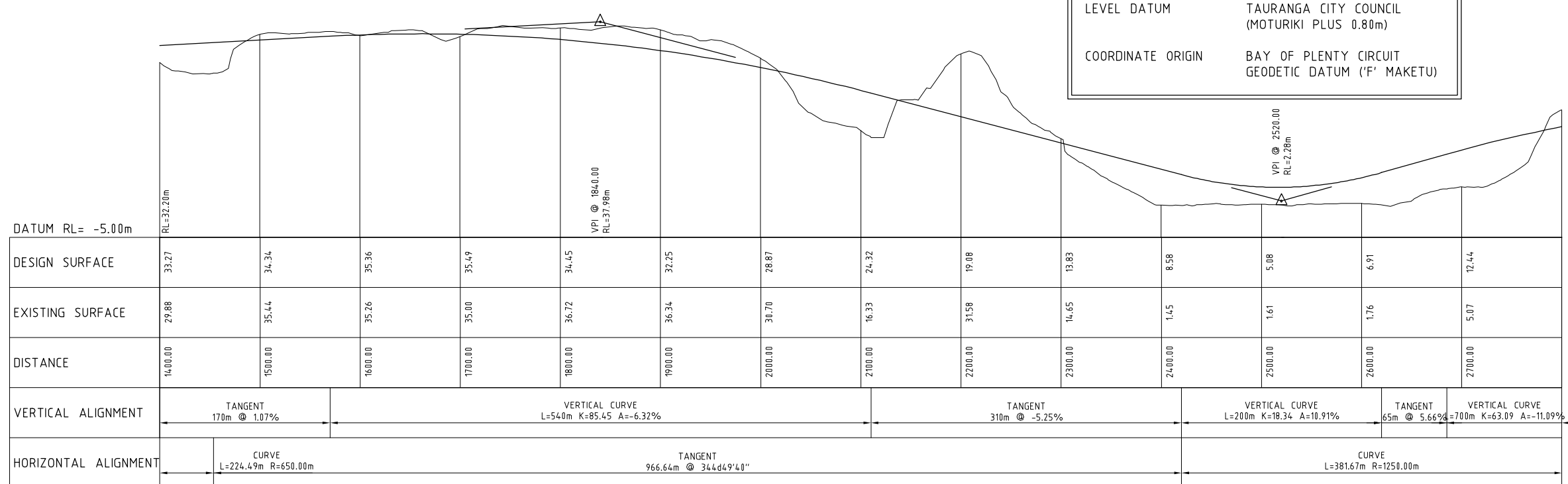
LONG SECTION HORIZONTAL SCALE 1:2500 VERTICAL SCALE 1:500
