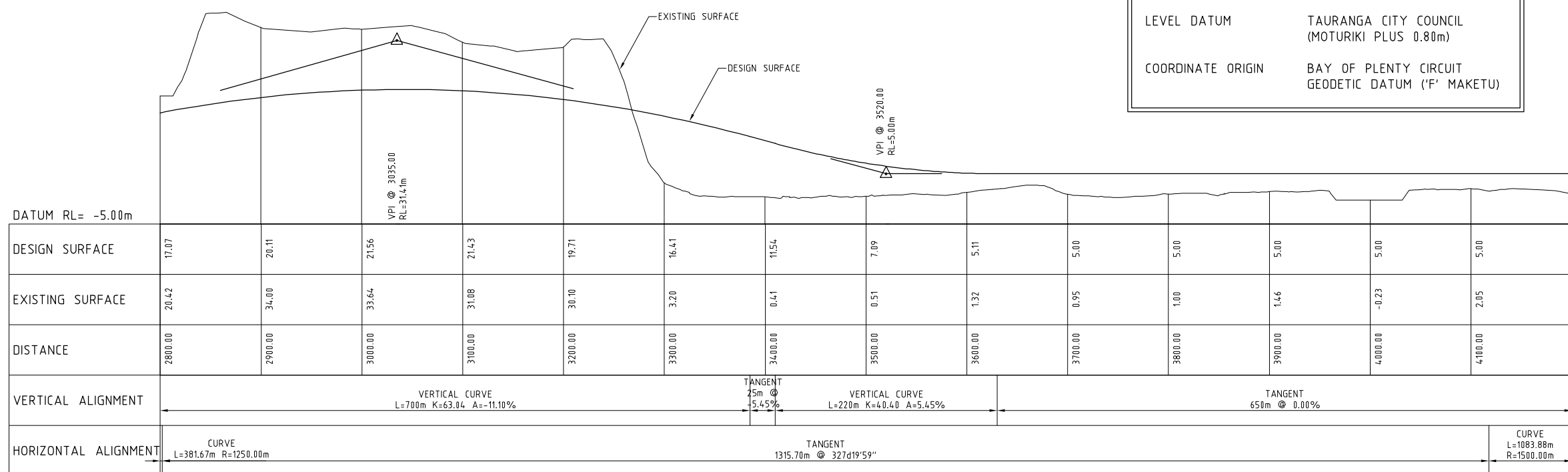
LONG SECTION HORIZONTAL SCALE 1:2500 VERTICAL SCALE 1:500
