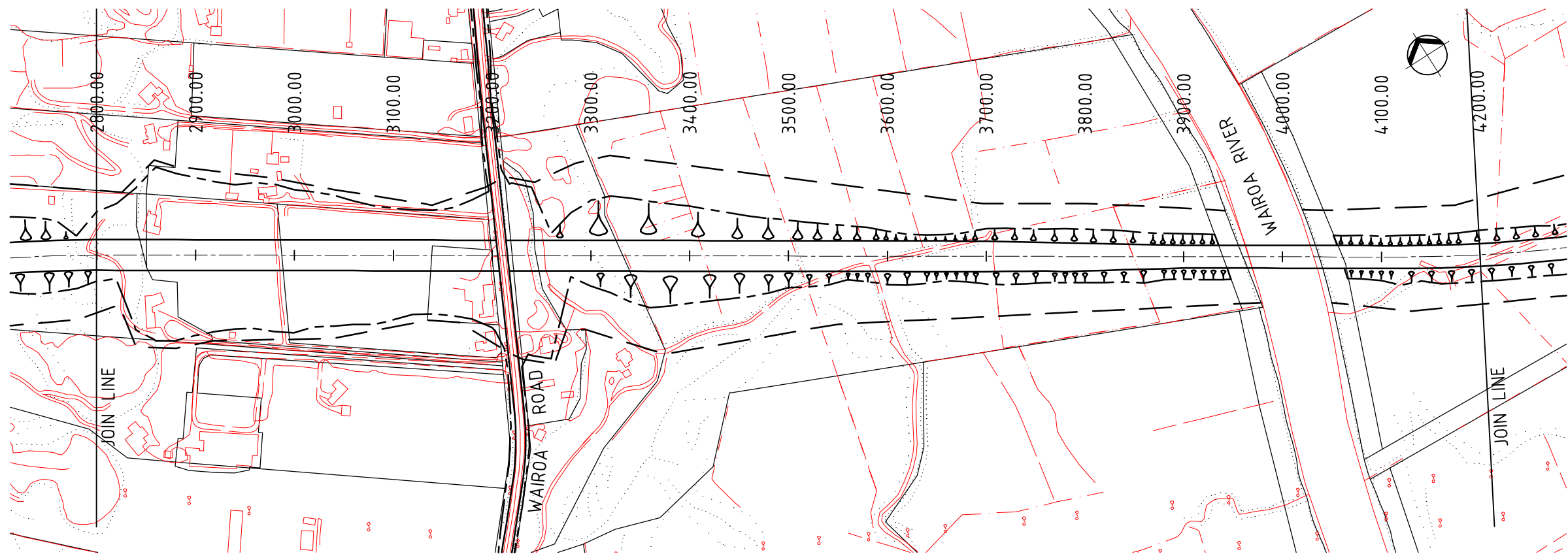
PLAN SCALE 1:2500
