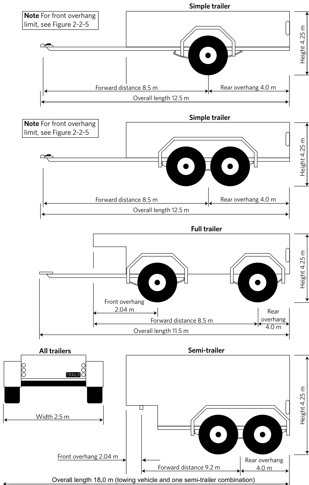
Figure 2-2-4. Trailer dimensions
