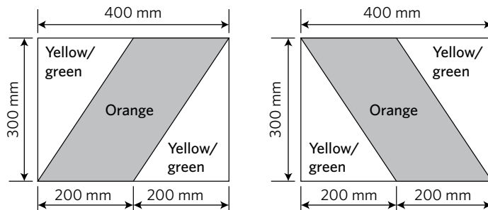
Figure 2-2-1. Hazard panel details
