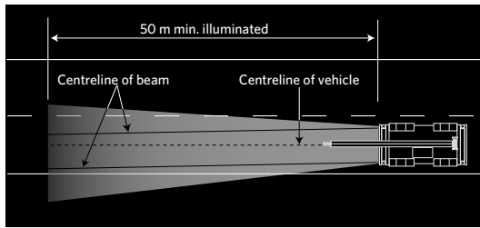
Figure 4-1-1. Minimum illuminated area
