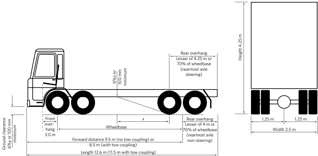
Figure 2-2-6. Dimensions for rigid heavy vehicles
