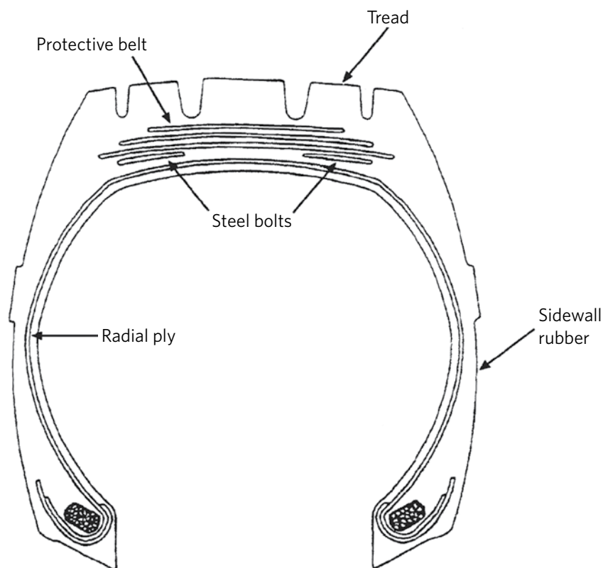
Figure 10-1-1. Cross-sectional representation of a heavy vehicleradial-ply tyre
