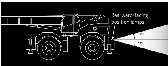
(a) Vertical beam angles
