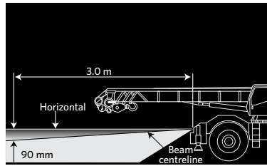
(b) Beam dip angle
