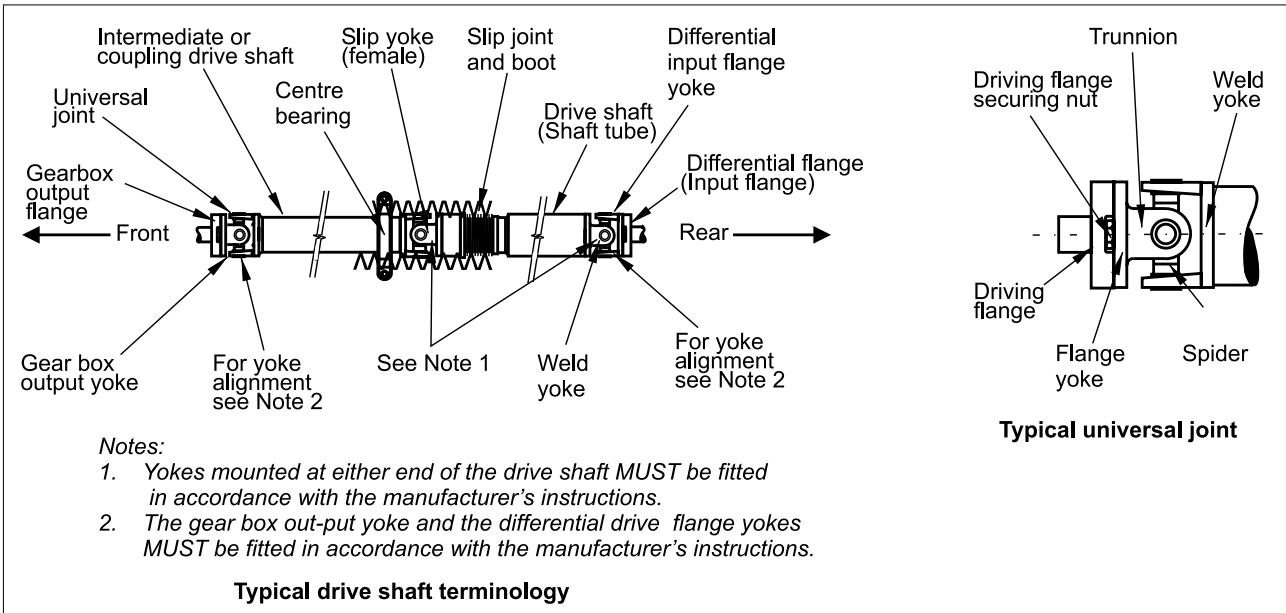
13-1-1. A typical driveshaft assembly
