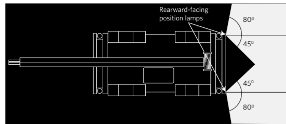
(b) Horizontal beam angles
