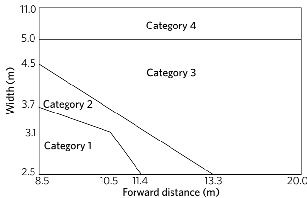
Figure 2-2-3. Overdimension vehicle categories for width/forward distance thresholds
