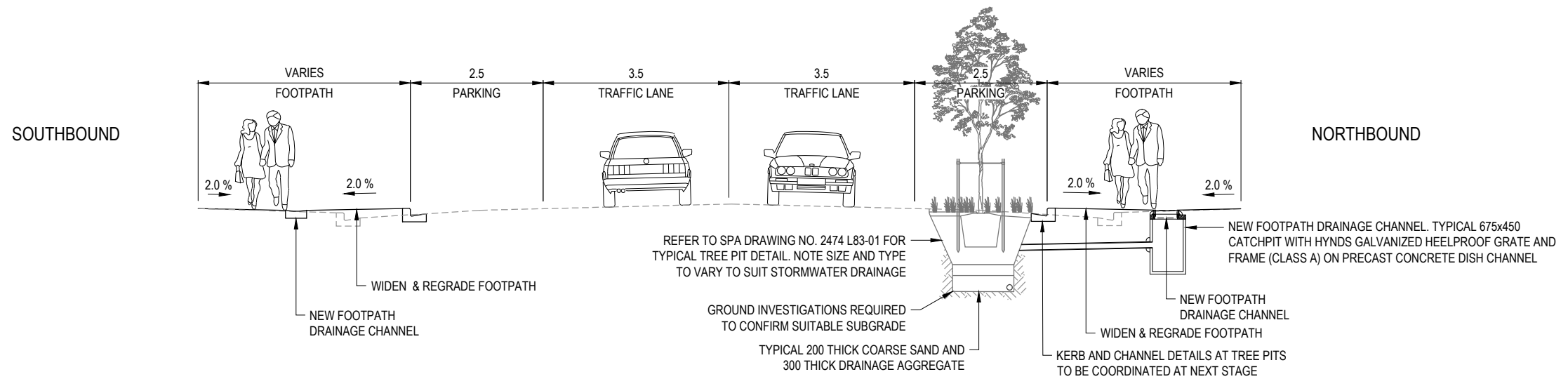
SECTION 6A 6A 6A PROPOSED SCALE 1:100 (205 206 406)
