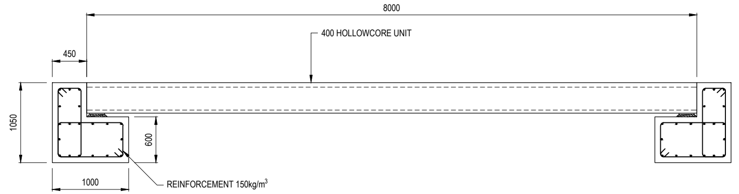
SECTION 1 OPTION 1 - CONCRETE SLAB BRIDGE (DESIGN LIFE 100 YEARS) SCALE 1:50
