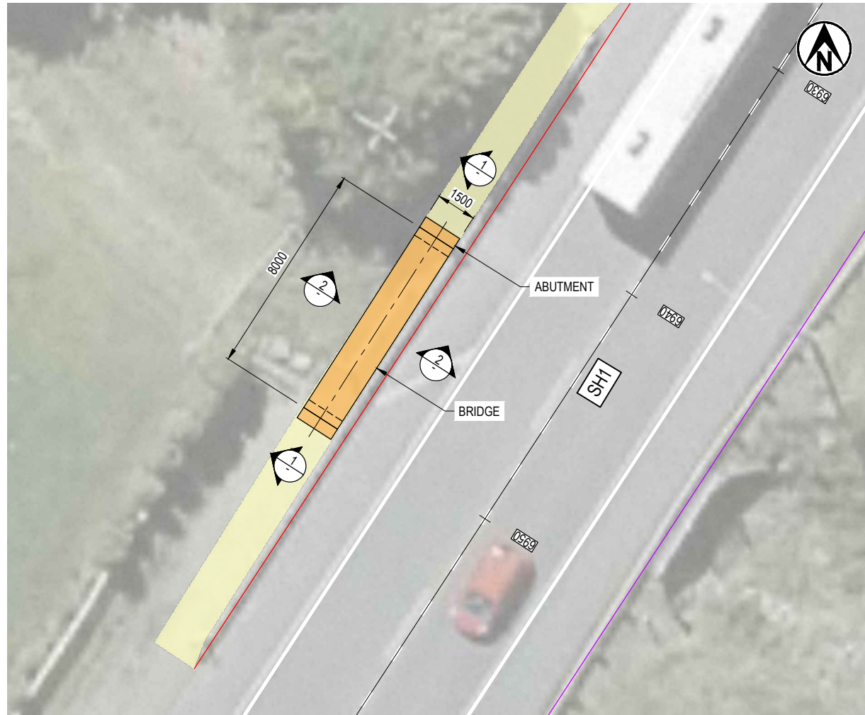
PLAN - SHARED PATH BRIDGE OVER EXISTING CULVERT / STREAM SCALE 1:200
