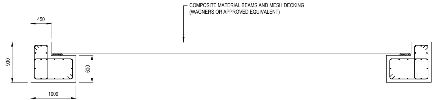
SECTION 1 OPTION 2 - COMPOSITE BRIDGE (DESIGN LIFE 100 YEARS) SCALE 1:50
