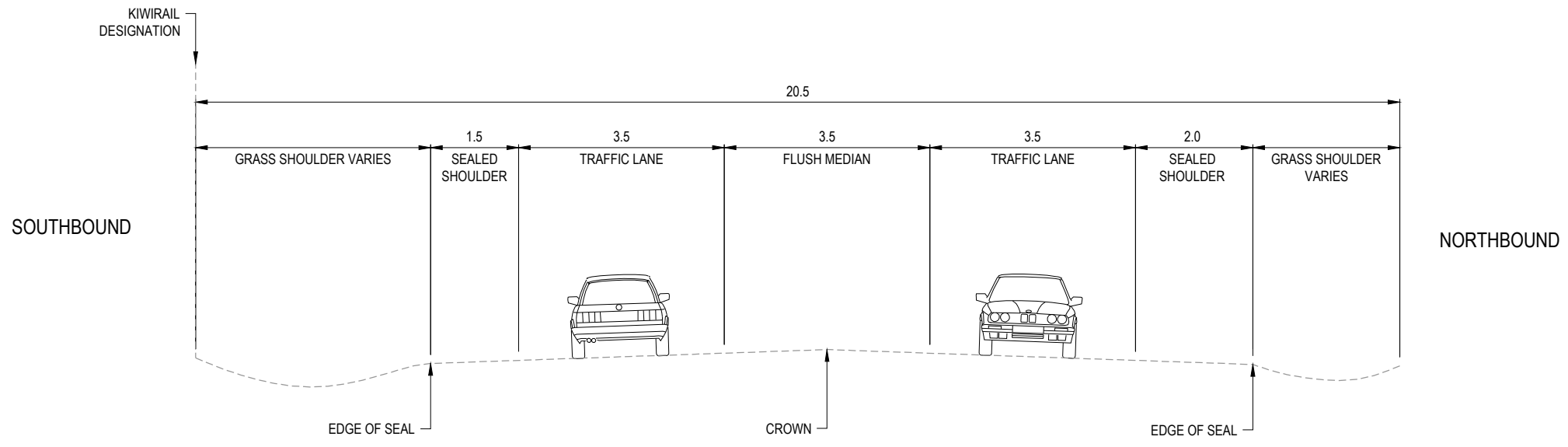
SECTION 11 11A EXISTING SCALE 1:100 221 223
