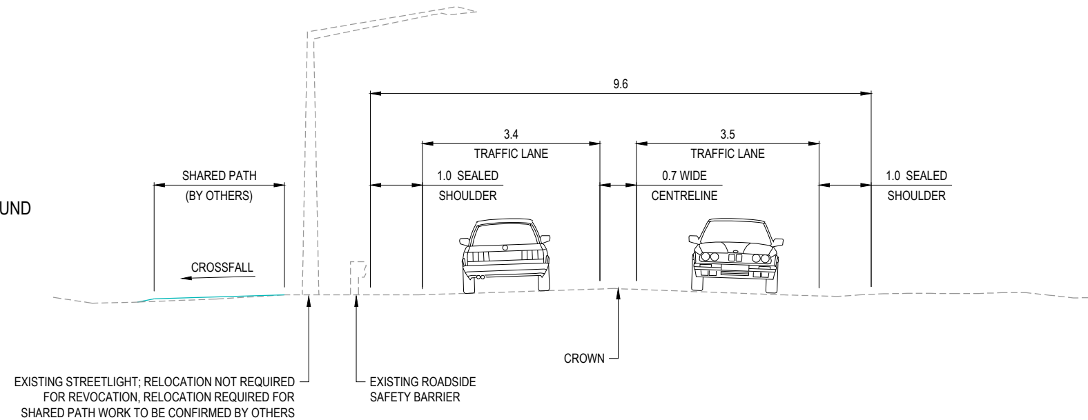
SECTION 3A PROPOSED SCALE 1:100
