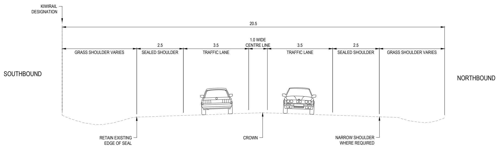
SECTION 11A 11A PROPOSED SCALE 1:100 221 223
