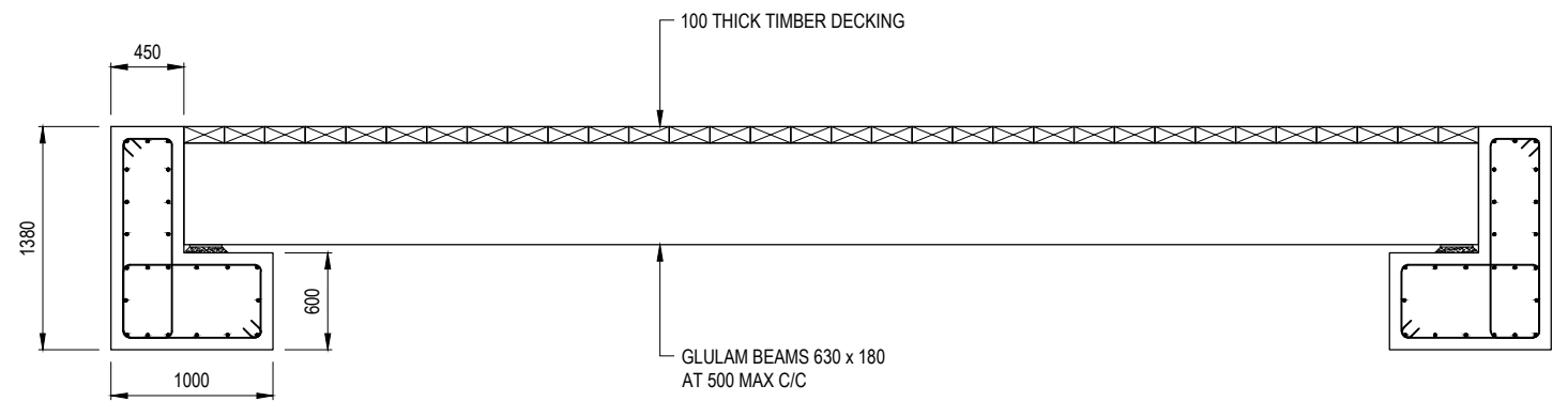
SECTION 1 OPTION 3 - TIMBER BRIDGE (DESIGN LIFE 50 YEARS) SCALE 1:50
