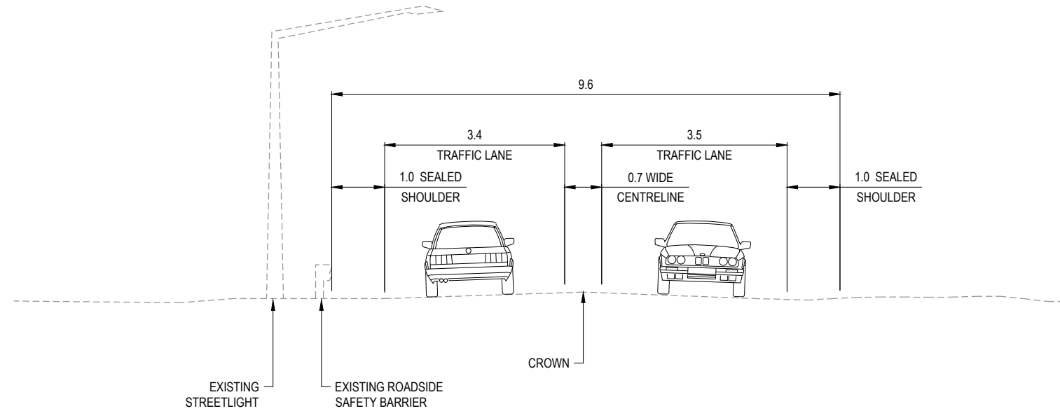
SECTION 3 EXISTING SCALE 1:100
